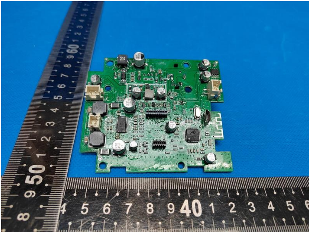
Inner View of the EUT
