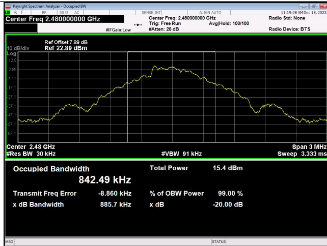
GFSK_DH1_Channel 78
