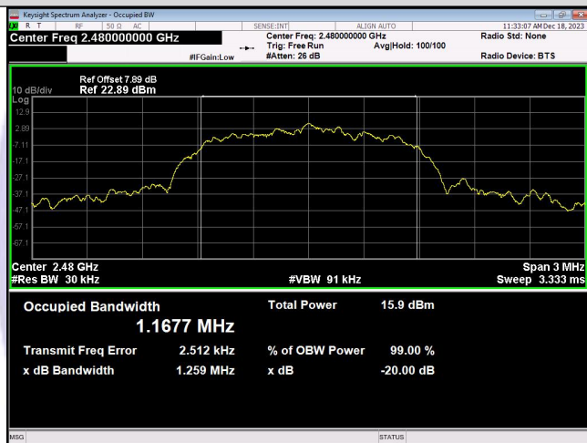
8DPSK_3-DH1_Channel 78
