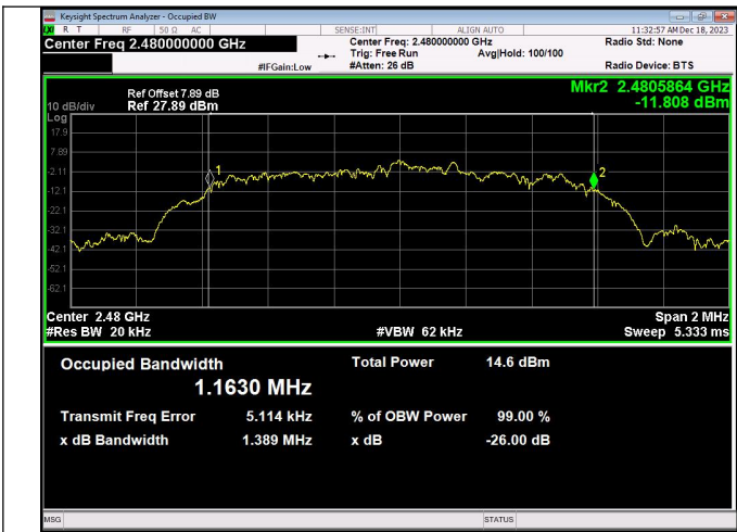
8DPSK_3-DH1_Channel 78
