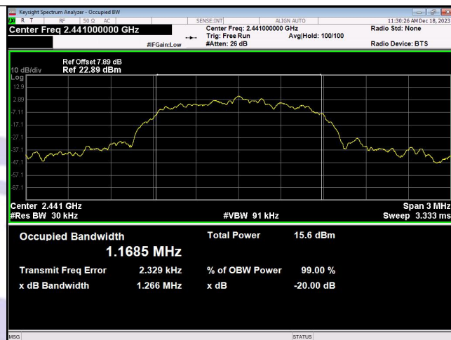
8DPSK_3-DH1_Channel 39
