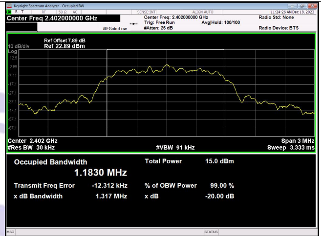
\pi/4 DQPSK_2-DH1_Channel 0
