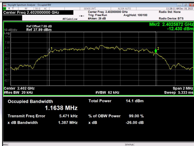
8DPSK_3-DH1_Channel 0
