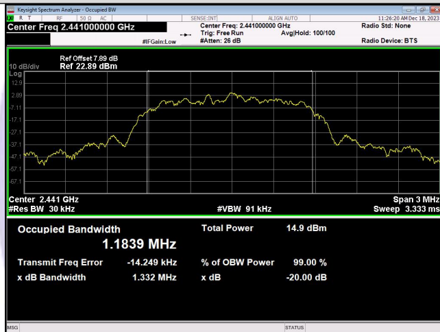
\pi/4 DQPSK_2-DH1_Channel 39
