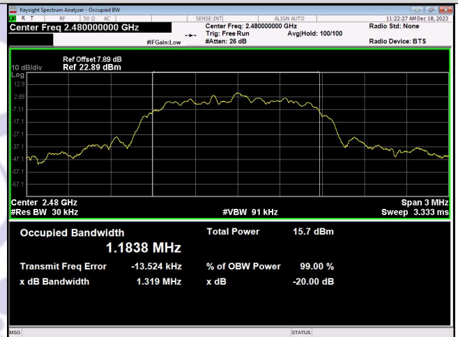
\pi/4 DQPSK_2-DH1_Channel 78
