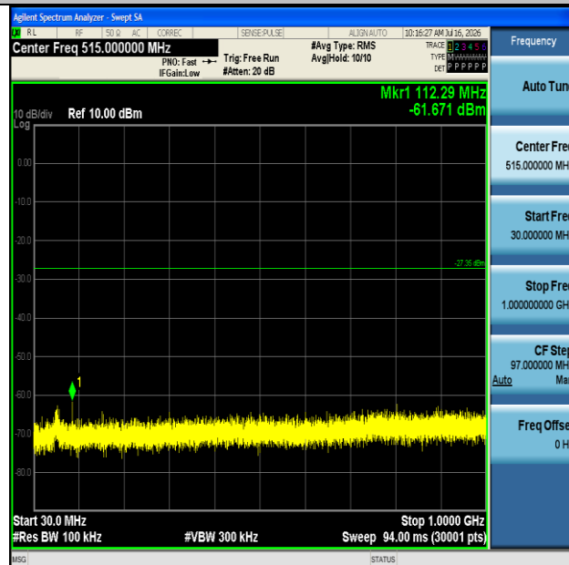
SRD-Ant1-2473-30~1000-PASS
