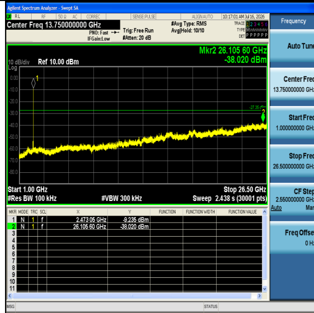
SRD-Ant1-2473-1000~26500-PASS
