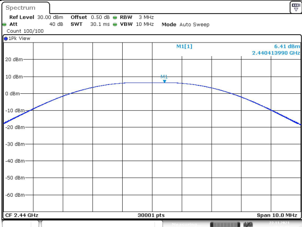
Channel 19 (2440MHz)
