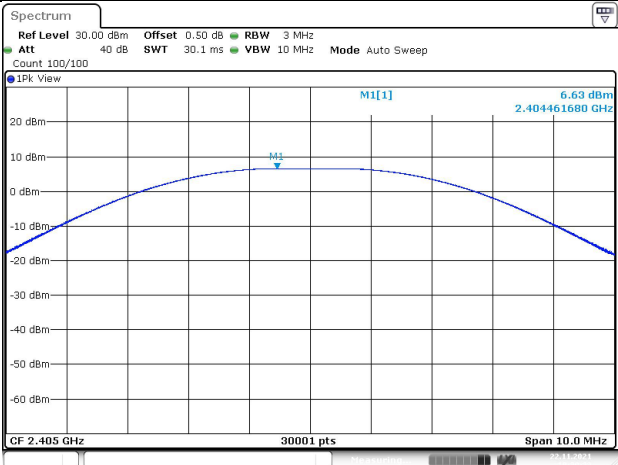
Channel 0 (2405MHz)
