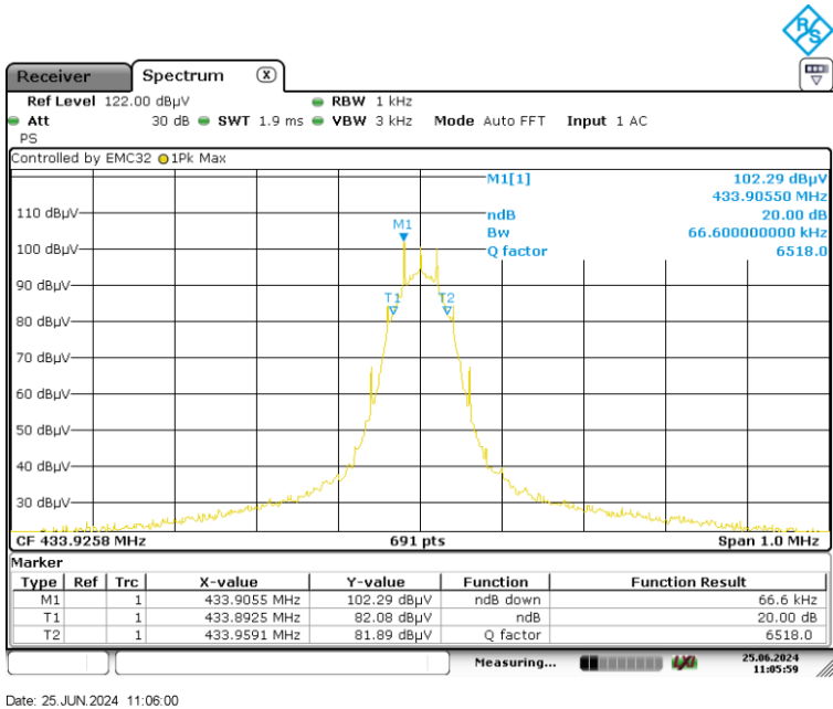
20dB Bandwidth
