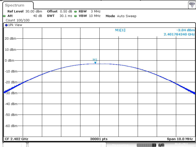
Channel 0 (2402MHz)
