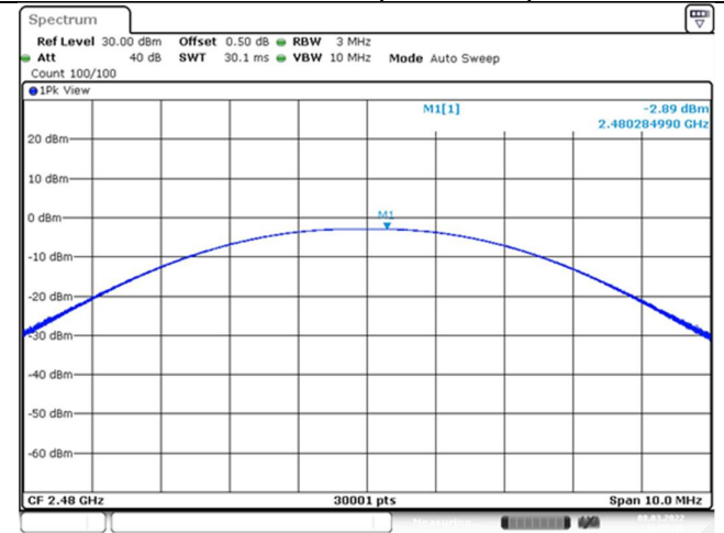
Channel 39 (2480MHz)
