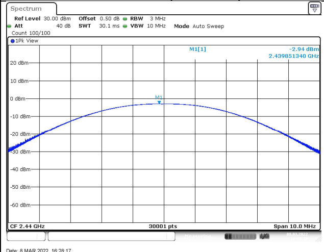
Channel 19 (2440MHz)
