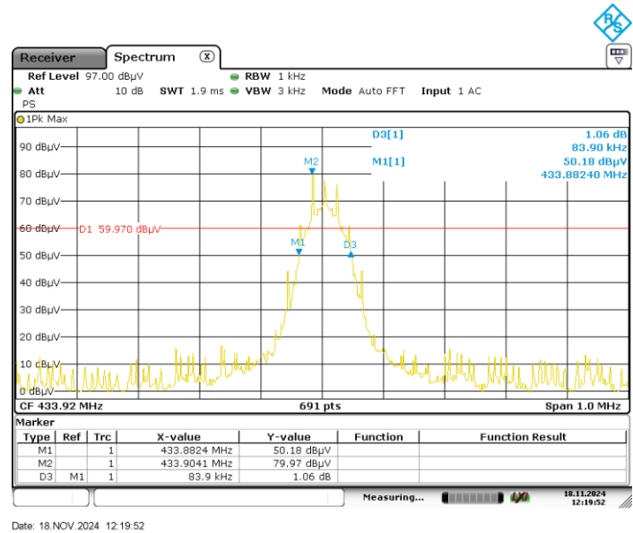
20dB Bandwidth
