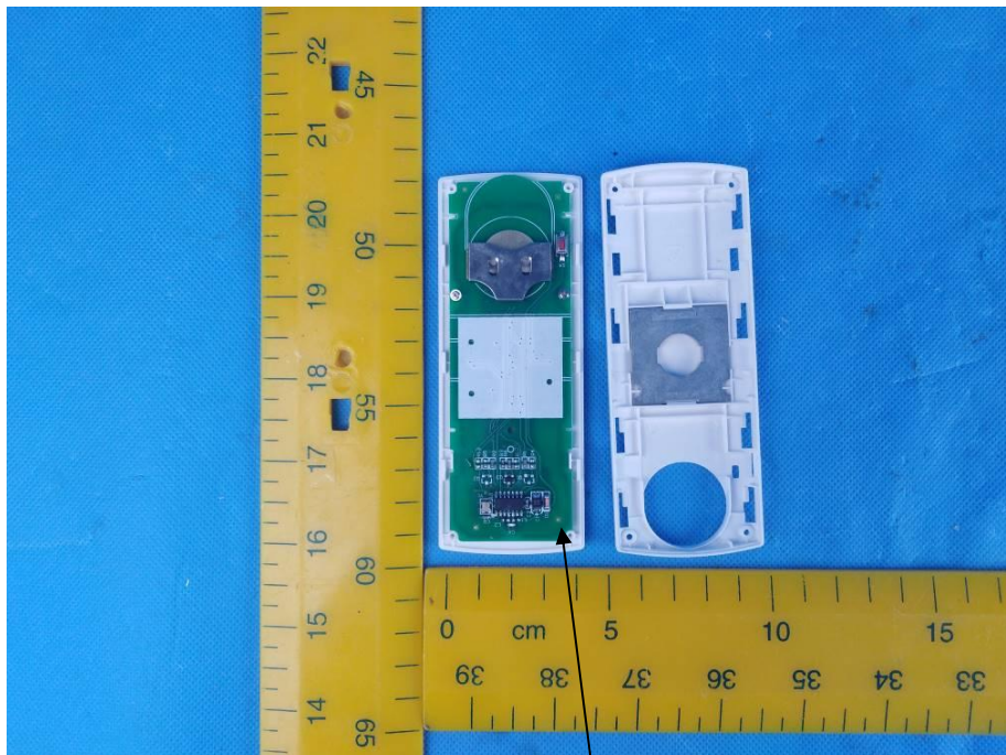
RF Antenna
