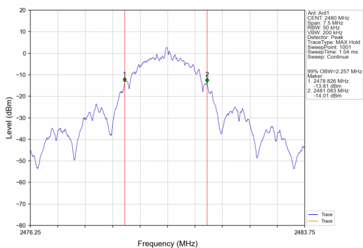
Thread_HCH_2480MHz_Ant1_NTNV
