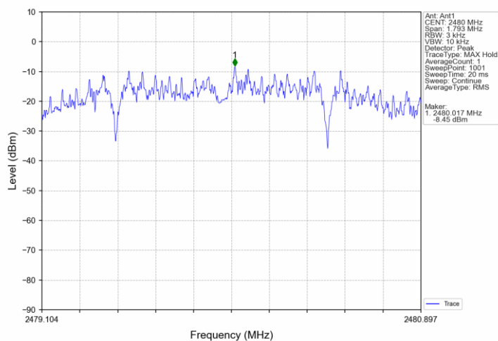
Thread_HCH_2480MHz_Ant1_NTNV
