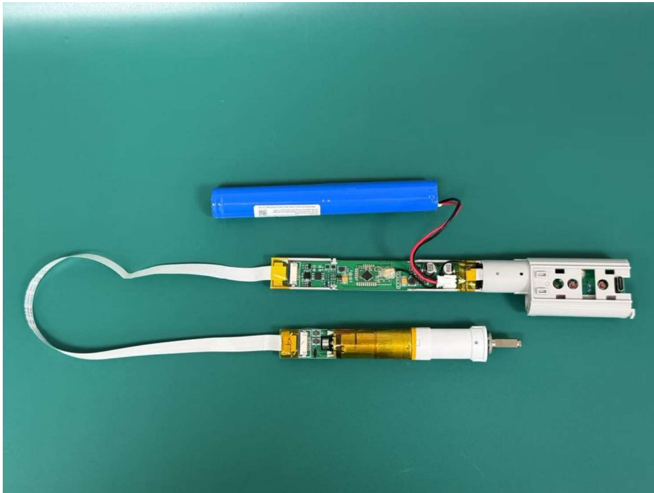
Internal: PCB
