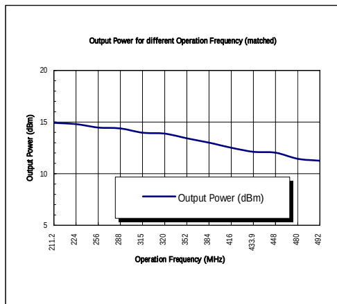
Figure 5. Output Power vs. Frequency
