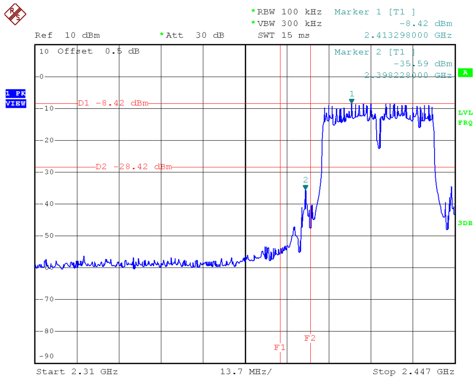
(Plot 2.6 D1: Channel = 3 @ 802.11n-40)
