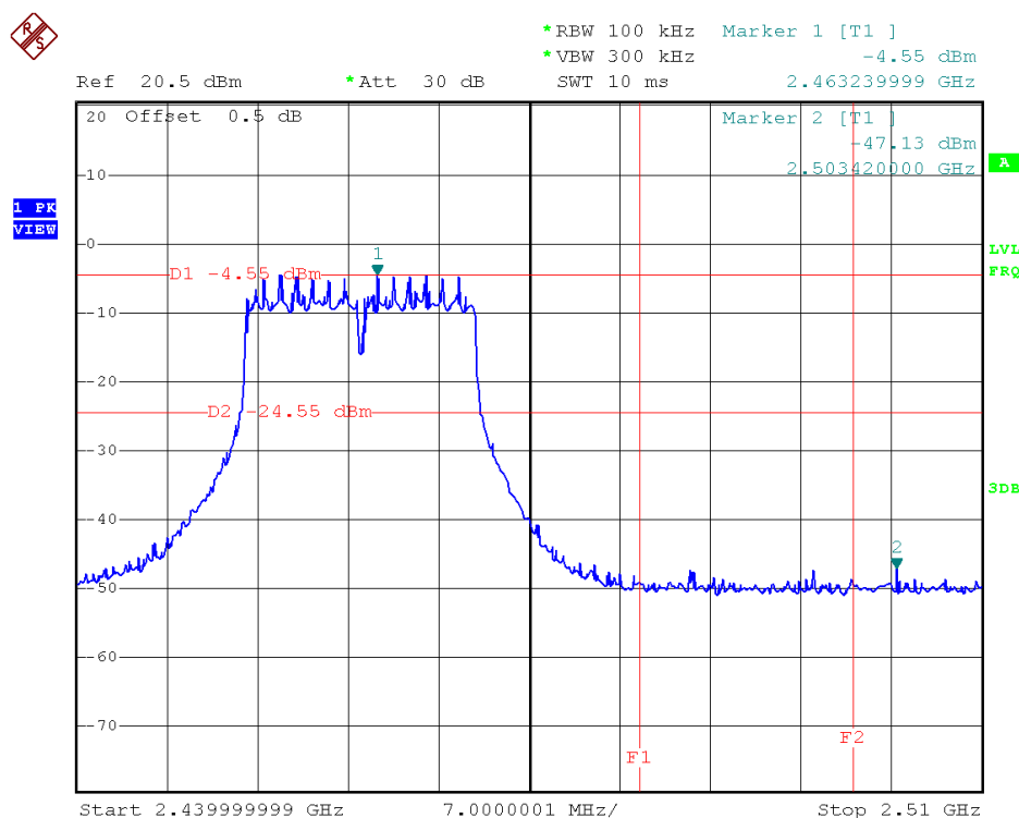
(Plot 2.6 C2: Channel = 11 @ 802.11n-20)
