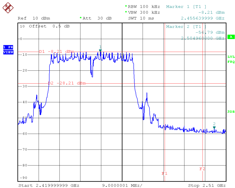
(Plot 2.6 D2: Channel = 9 @ 802.11n-40)
