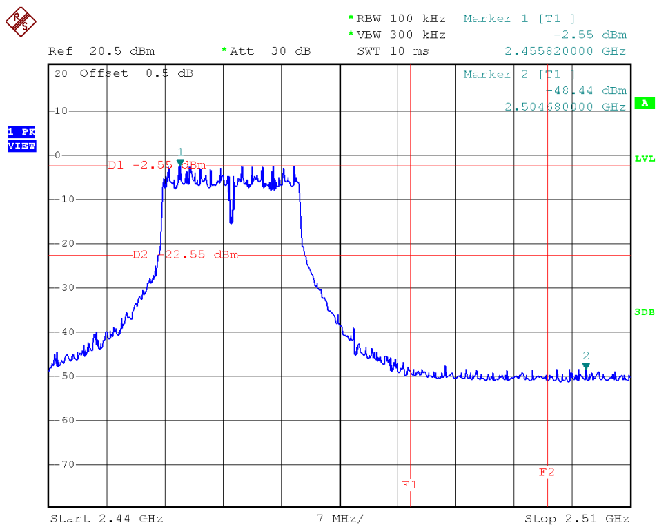
(Plot 2.6 B2: Channel = 11 @ 802.11g)
