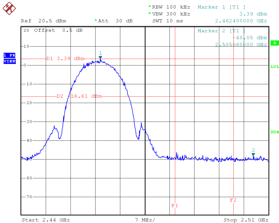
(Plot 2.6 A2: Channel = 11 @ 802.11b)
