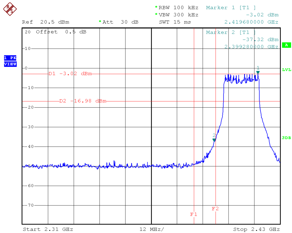
(Plot 2.6 B1: Channel = 1 @ 802.11g)
