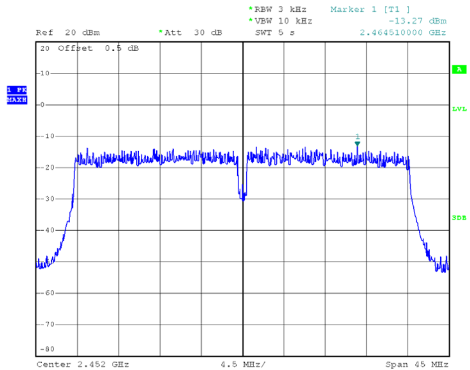
802.11n40 - Channel 9
