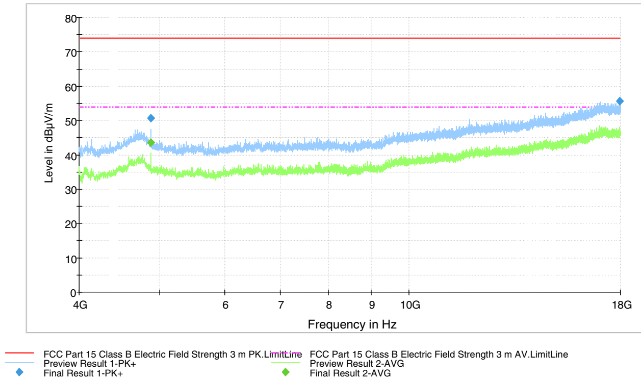
Figure 19. Measured curve with peak- and average detector (middle channel).
