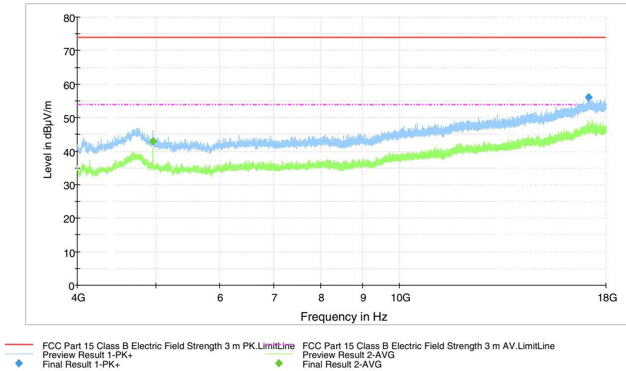
Figure 20. Measured curve with peak- and average detector (high channel).
