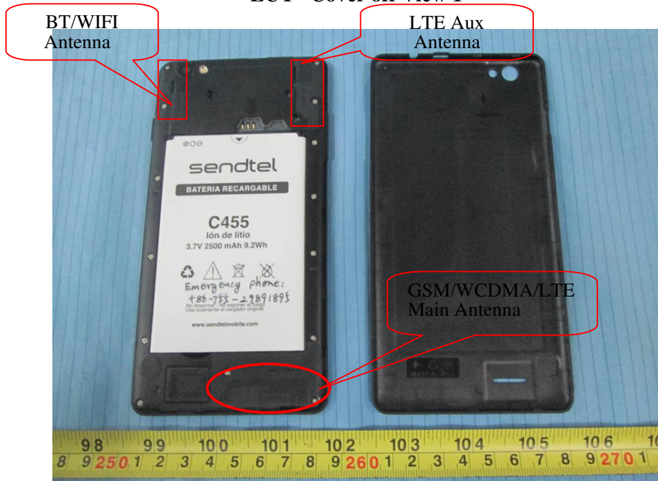
EUT -Cover off View 1
