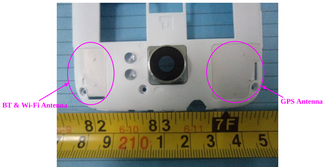
EUT – BT & Wi-Fi & GPS Antenna Location View
