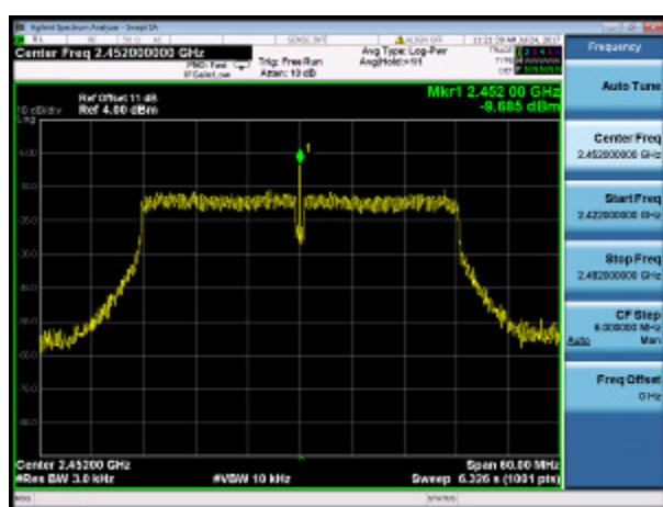
Channel 9 (2452MHz)
