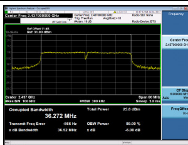
Channel 6 (2437MHz)
