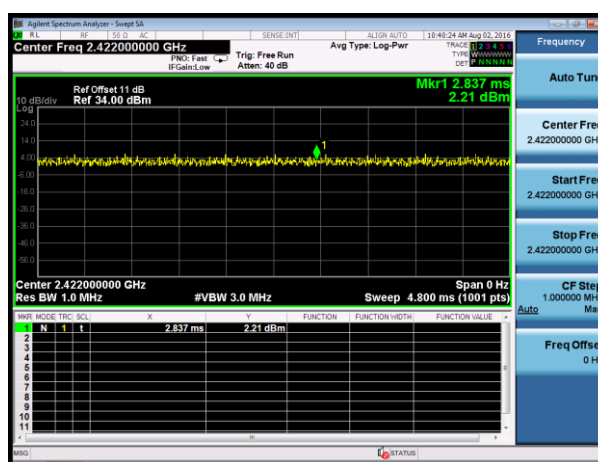
Transmit at 2422MHz by 802.11 n(40MHz)
