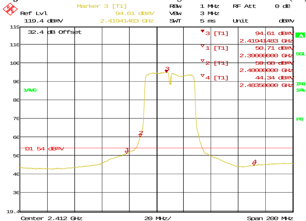
Figure 90: Radiated Emission at the Edge for 2390 MHz – Horiz. (Ave)
