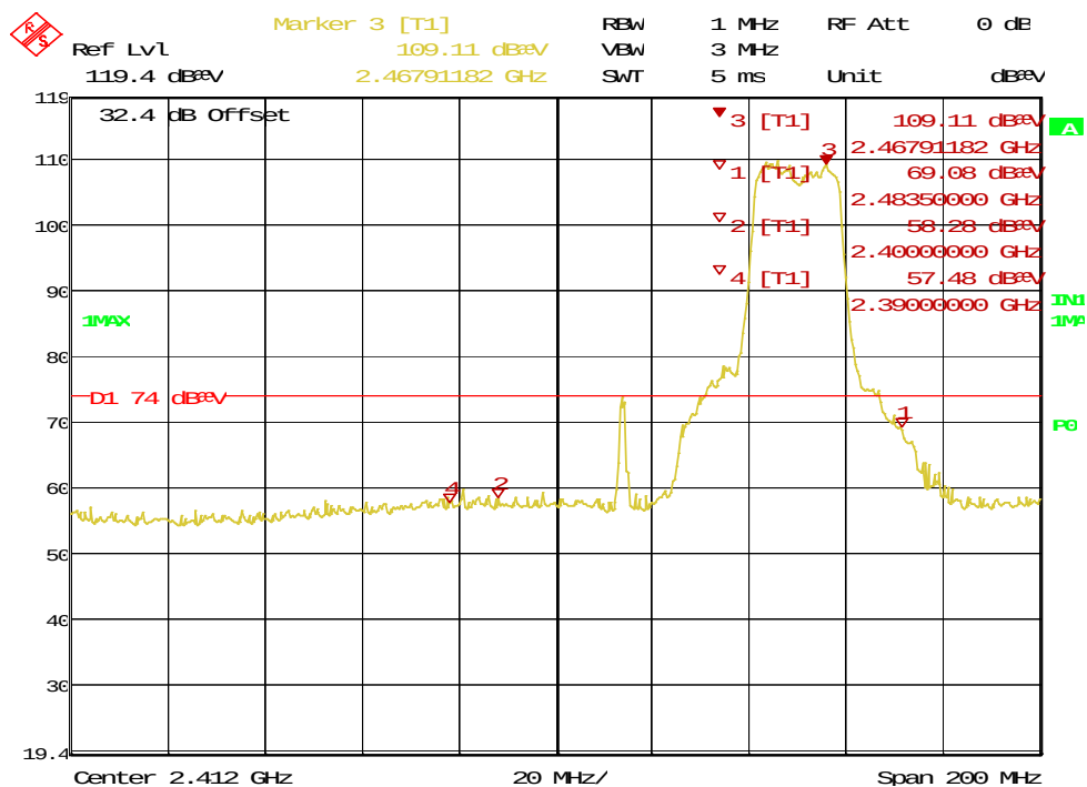
Figure 75: Radiated Emission at the Edge for 2483.5 MHz – Horz. (Pk)
