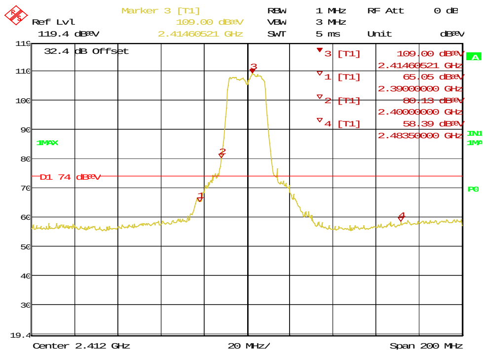
Figure 73: Radiated Emission at the Edge for 2390 MHz – Horz. (Pk)
