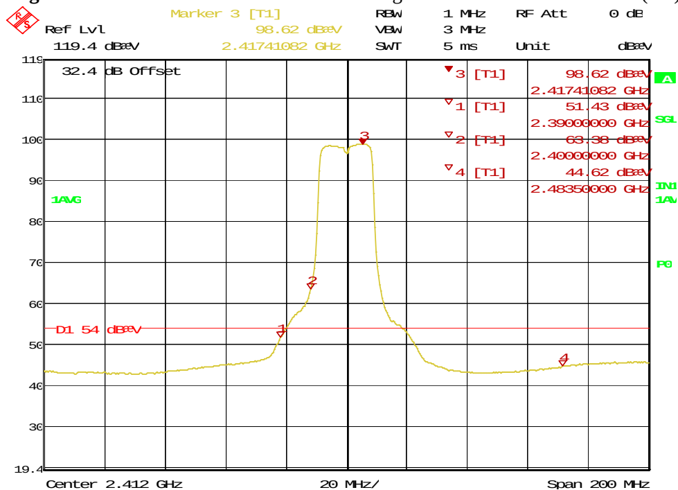
Figure 74: Radiated Emission at the Edge for 2390 MHz – Horz. (Ave)
