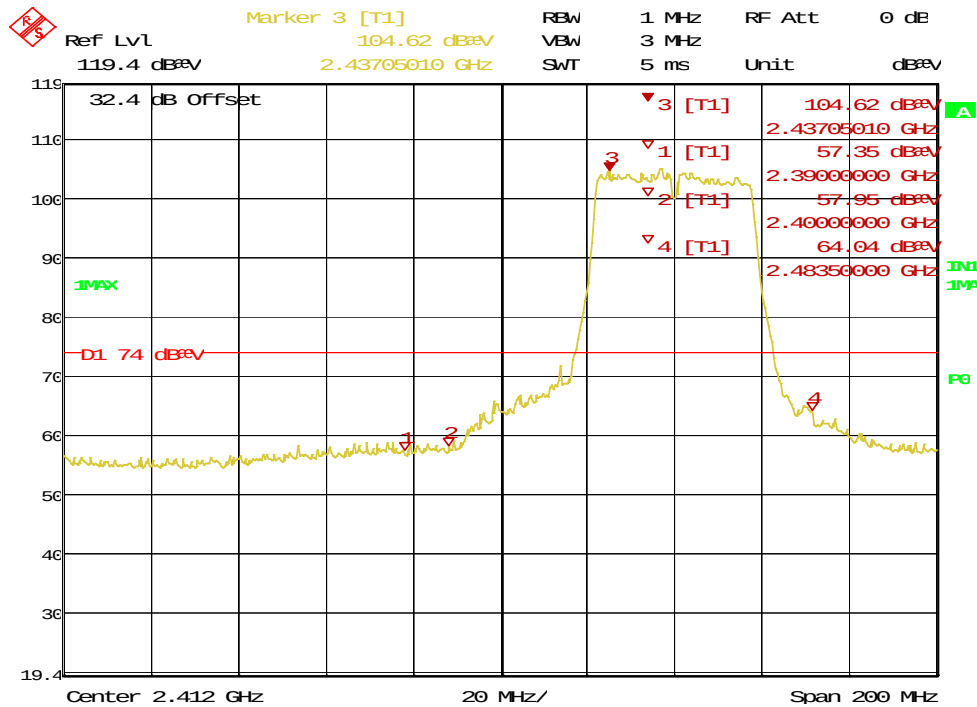
Figure 91: Radiated Emission at the Edge for 2483.5 MHz – Horiz. (Pk)
