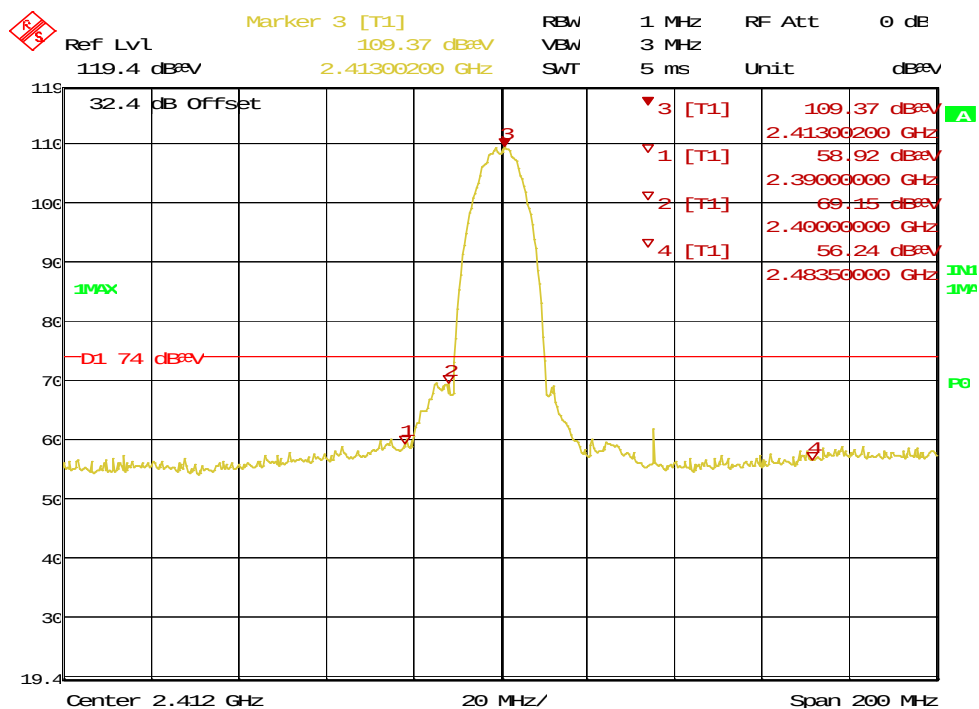
Figure 57: Radiated Emission at the Edge for 2390 MHz – Horz. (Pk)
