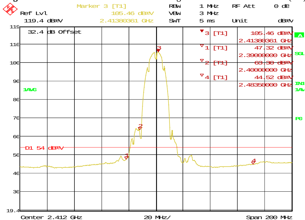
Figure 58: Radiated Emission at the Edge for 2390 MHz – Horz. (Ave)
