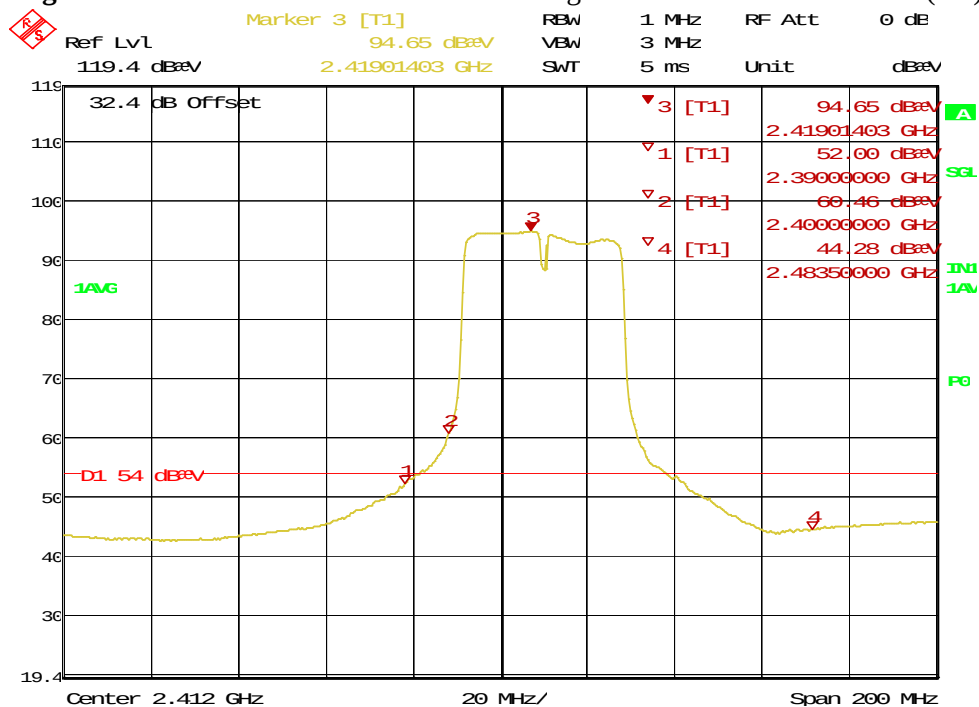
Figure 80: Radiated Emission at the Edge for 2390 MHz – Horiz. (Ave)
