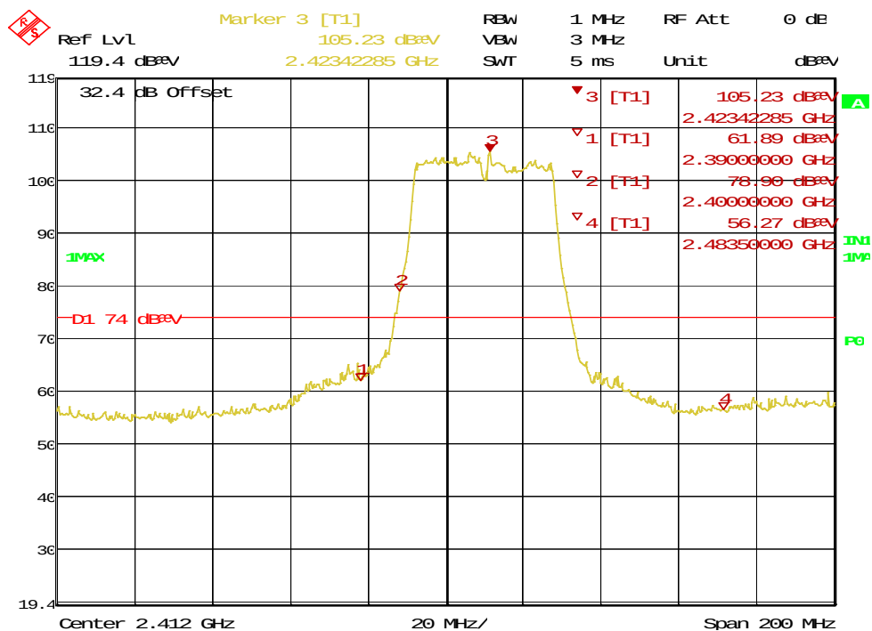
Figure 89: Radiated Emission at the Edge for 2390 MHz – Horiz. (Pk)
