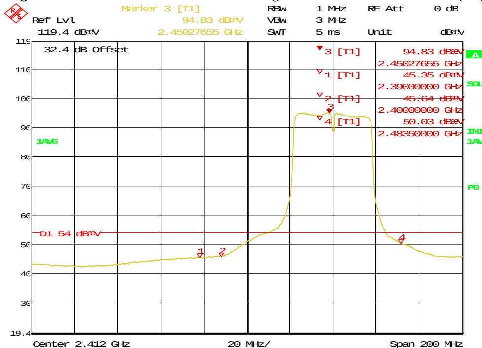
Figure 92: Radiated Emission at the Edge for 2483.5 MHz – Horiz. (Ave)
