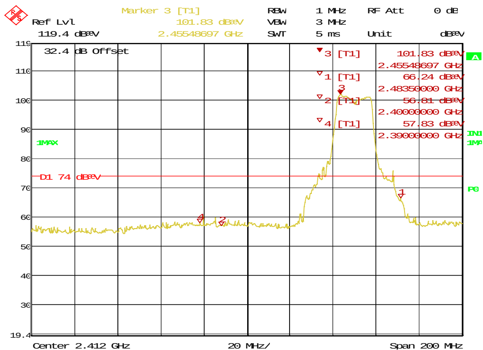
Figure 69: Radiated Emission at the Edge for 2483.5 MHz – Vert. (Pk)
