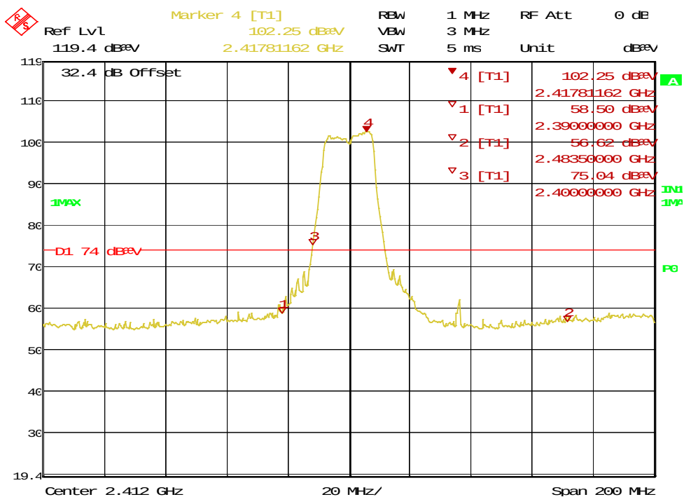
Figure 63: Radiated Emission at the Edge for 2390 MHz – Vert. (Pk)
