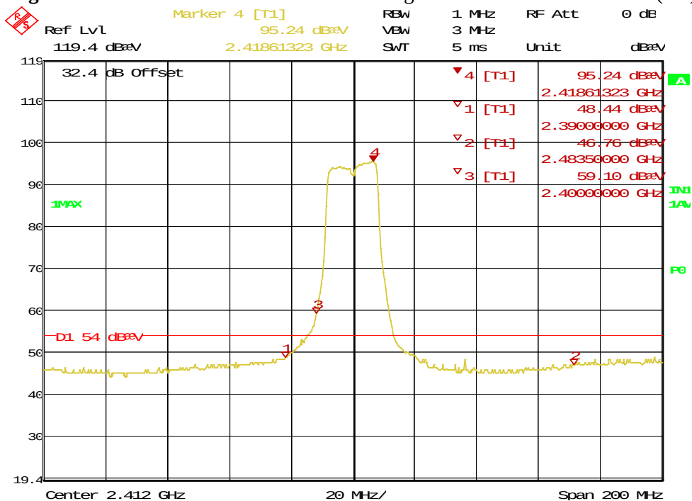
Figure 64: Radiated Emission at the Edge for 2390 MHz – Vert. (Ave)
