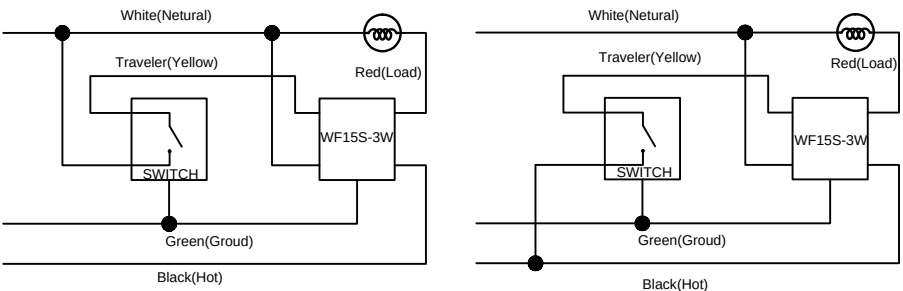
Wiring Method 1
