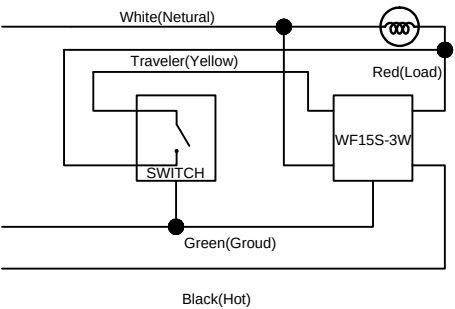
Wiring Method 3
