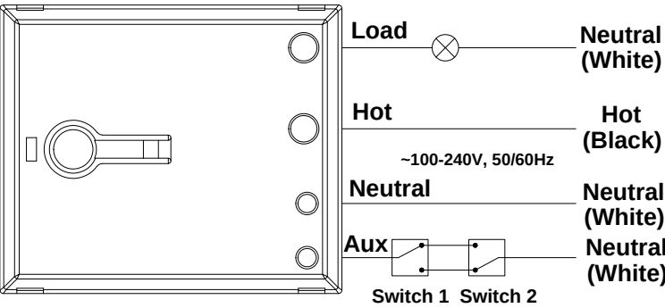
3-way Circuits Wiring Diagram: Fig2
