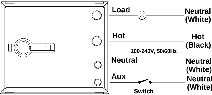
3-way Circuits Wiring Diagram: Fig2
