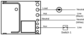
Wiring Diagram 2:
