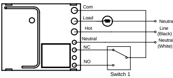
Wiring Diagram 1:
