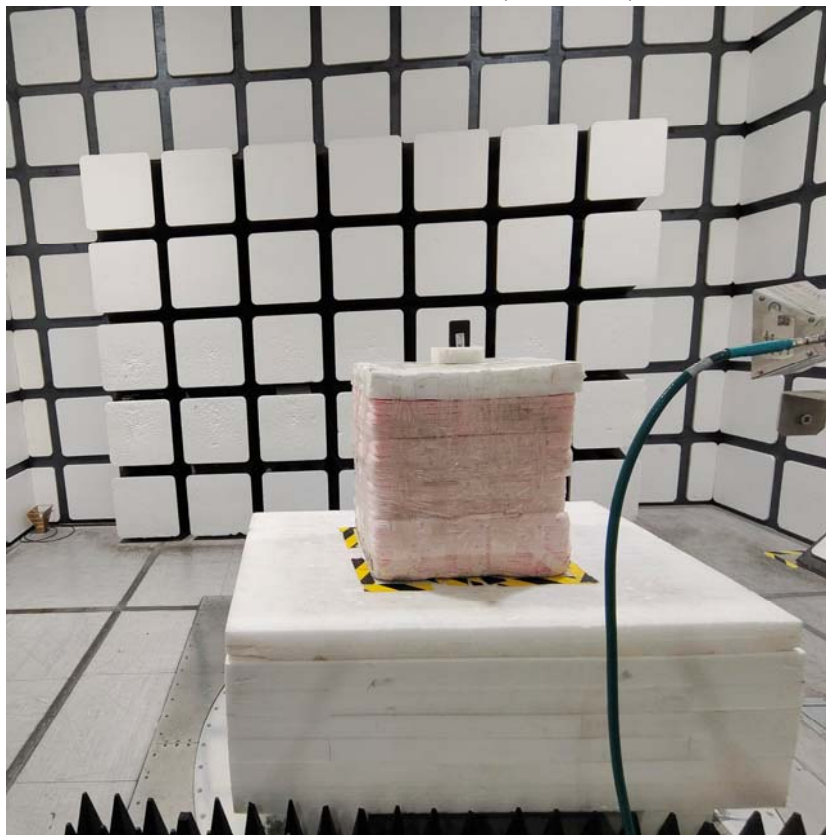
Radiated Emissions View (18-40 GHz)
