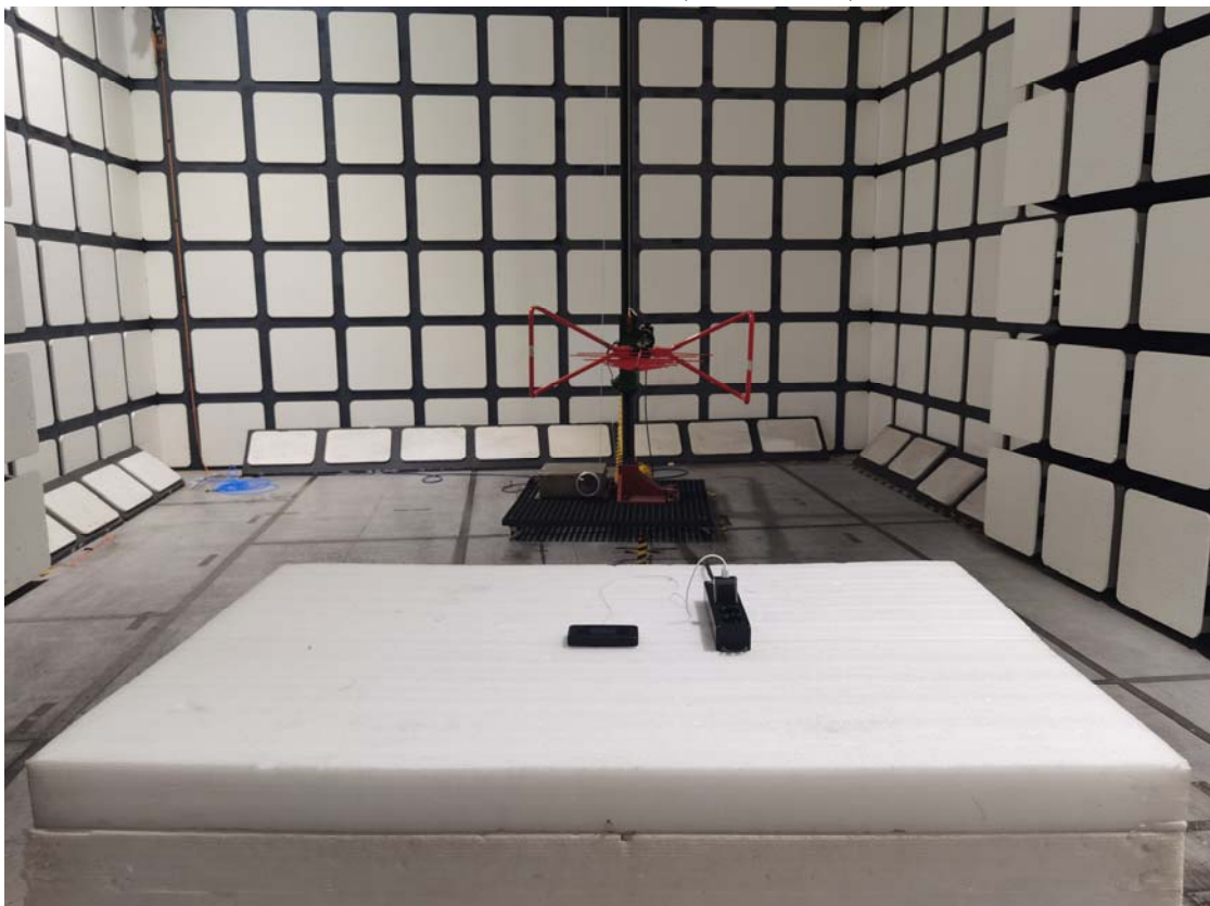
Radiated Emissions View (Below 1 GHz)
