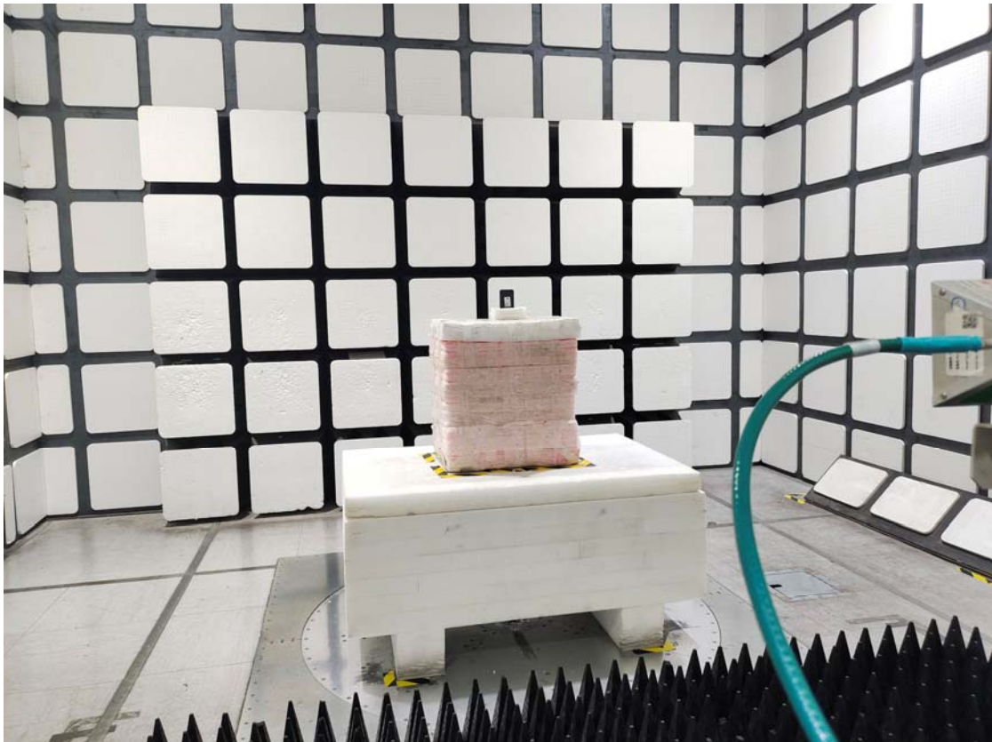
Radiated Emissions View (18-25 GHz)
