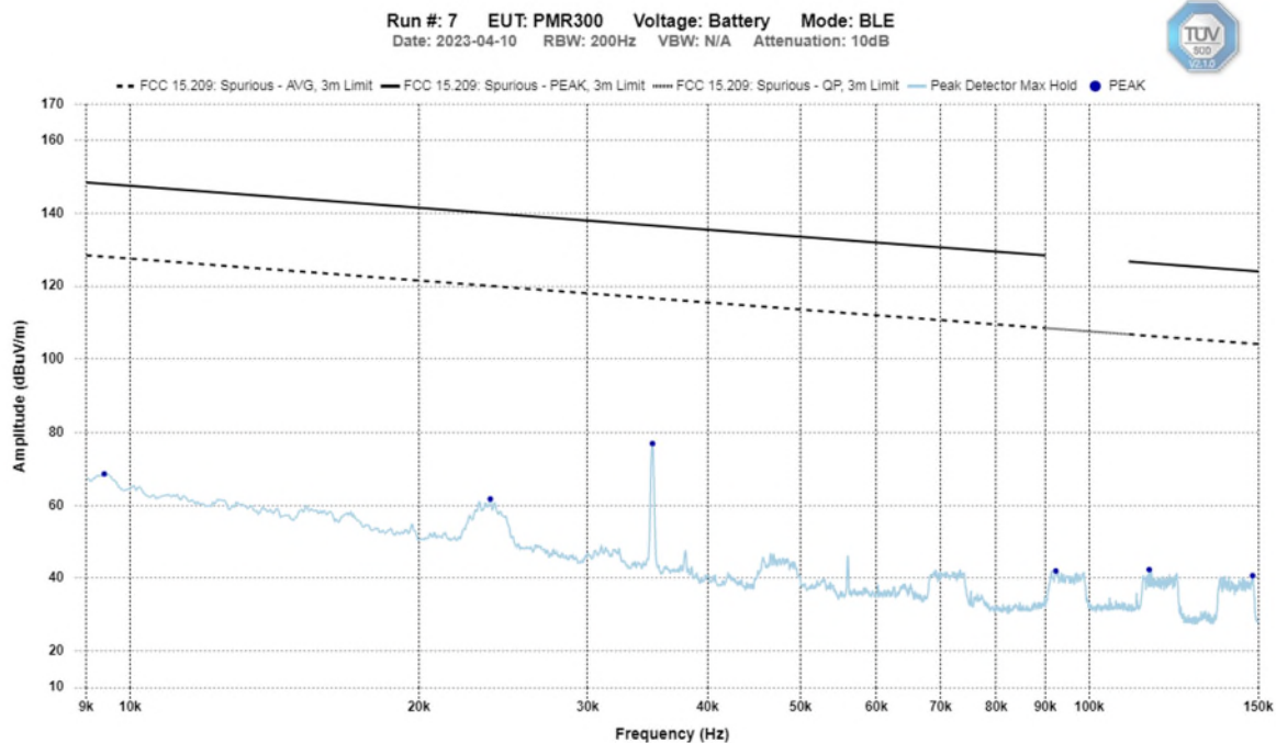
High Channel - 9 kHz – 150 kHz Peak Emission Graph
