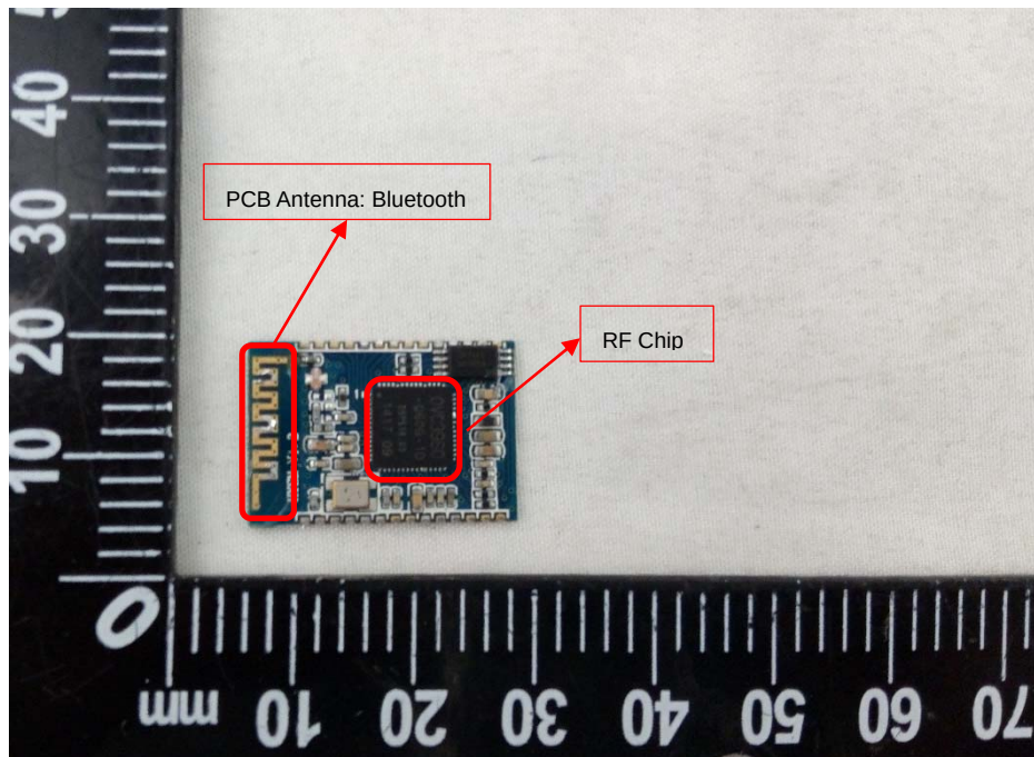
MAIN BOARD 2 FRONT VIEW
