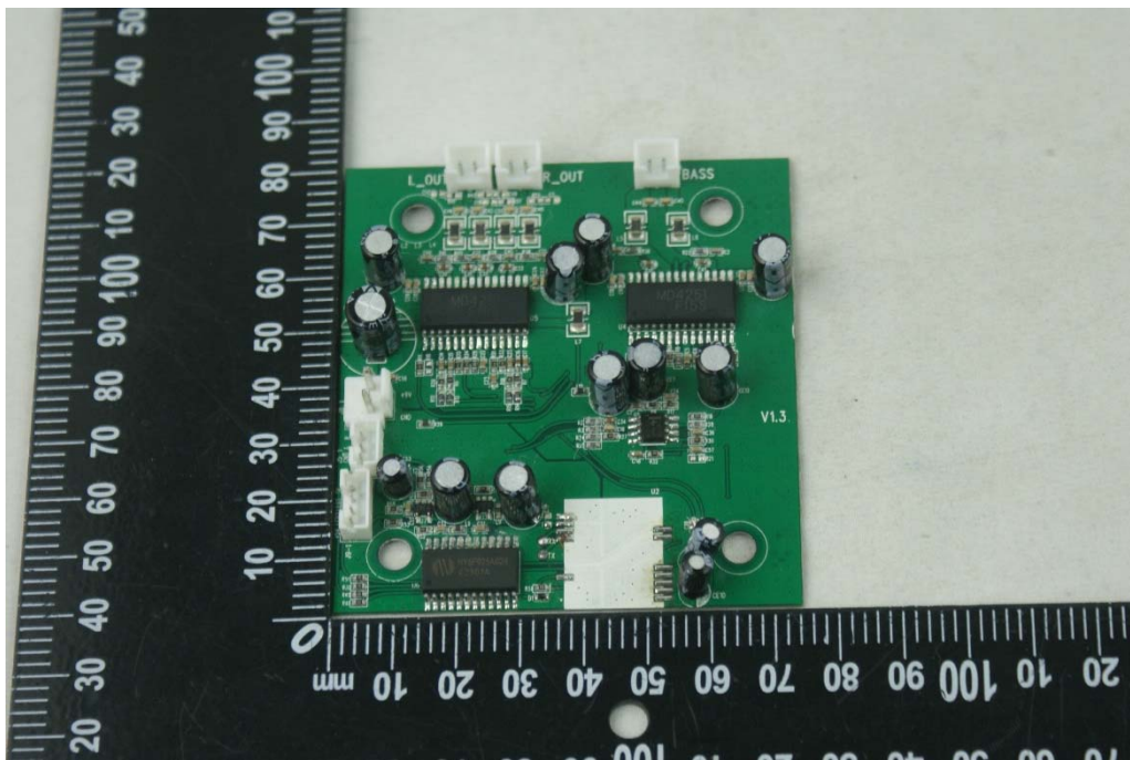
MAIN BOARD 3 FRONT VIEW
