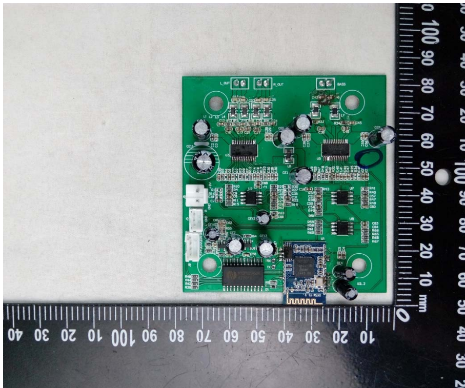
MAIN BOARD 1 FRONT VIEW
