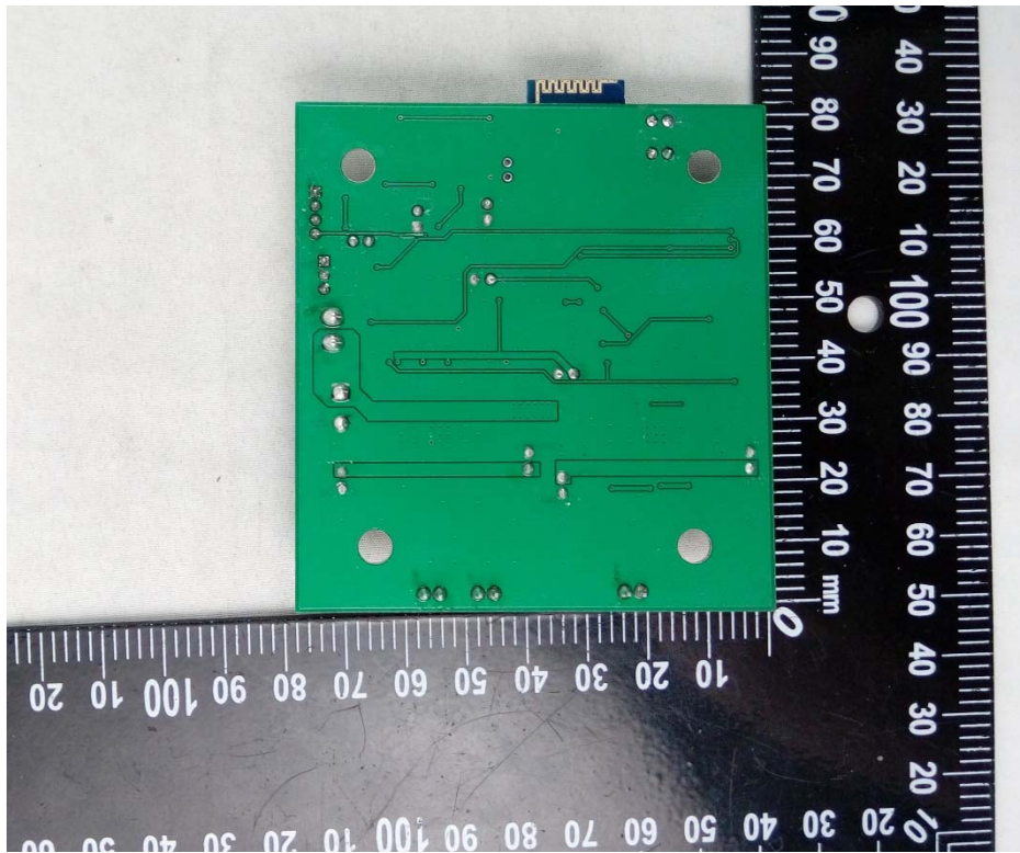
MAIN BOARD 1 REAR VIEW
