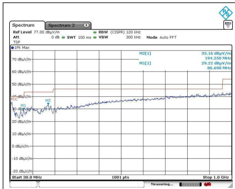
Aux-in and charging mode, 30MHz – 1GHz, Vertical
