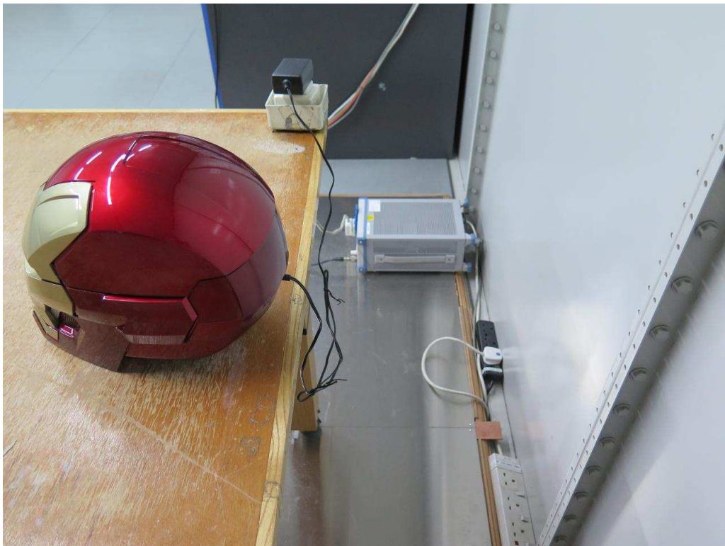
Side view, Line-conducted emission
