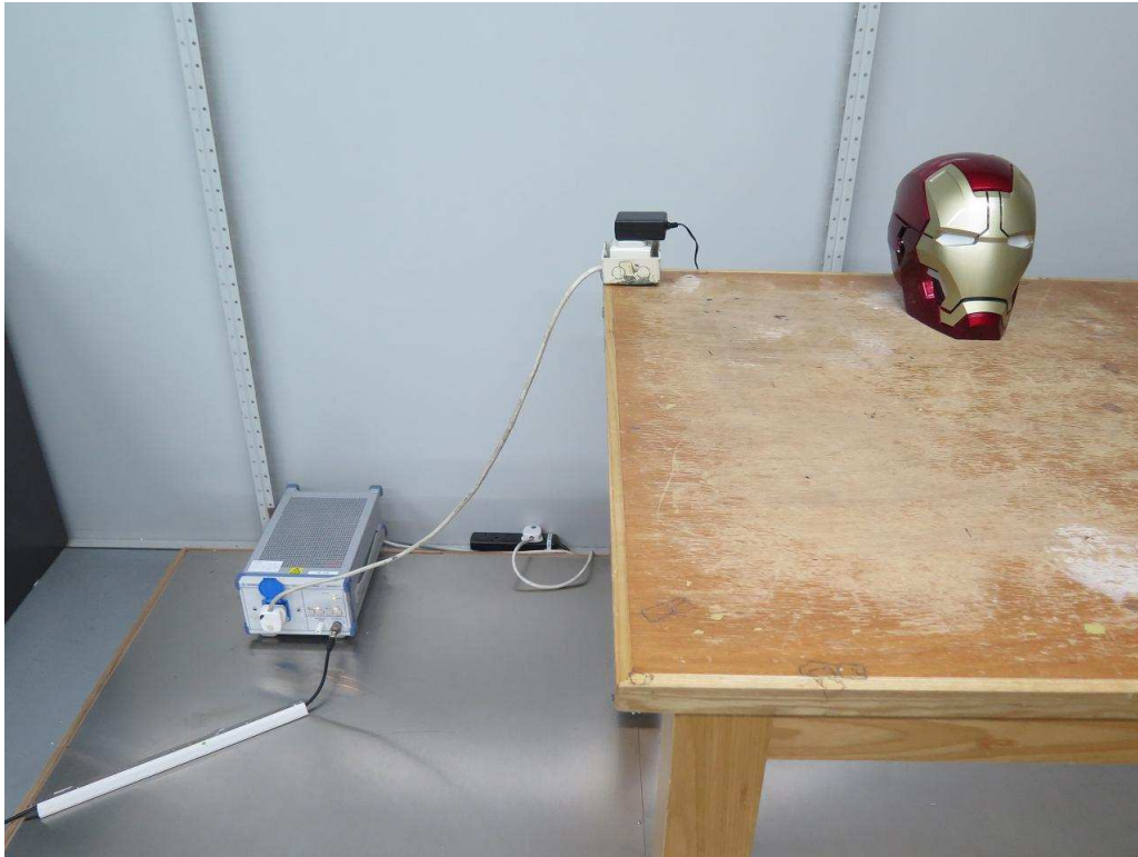
Front view, Line-conducted emission
