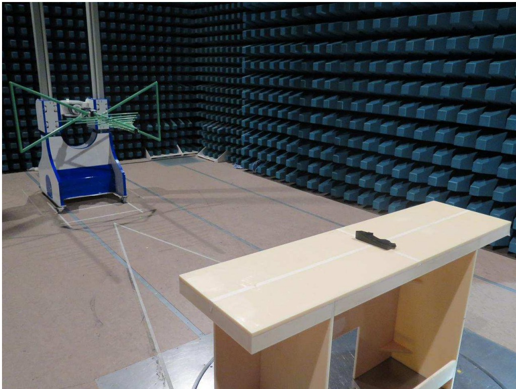
LED on
