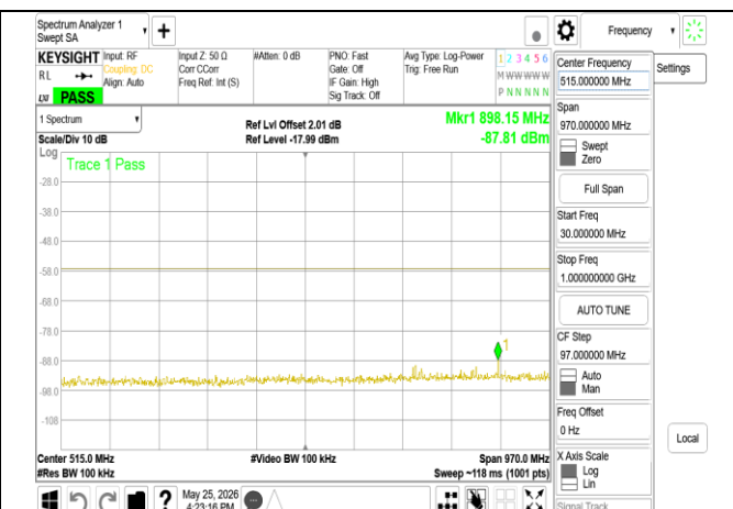
LPI_802.11be_160MHz_Chain0_6345MHz_Range1
