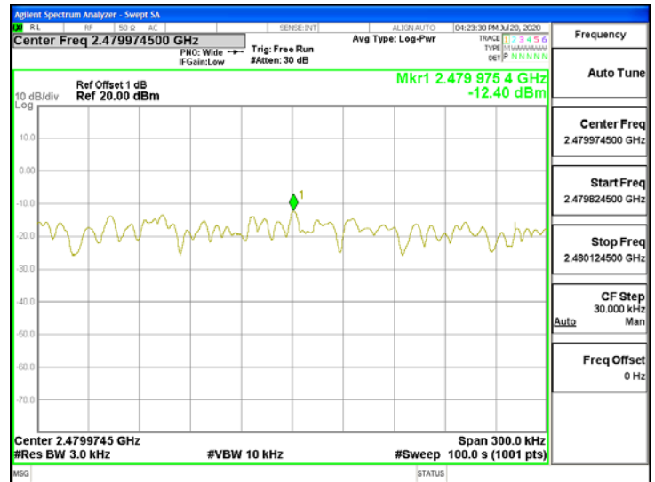
功率密度_BLE_1M_HighCH39-2480
