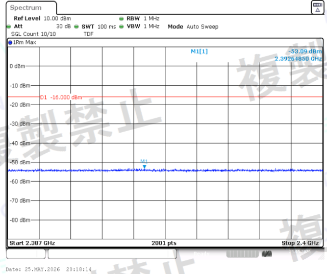
NTNV-BLE_1M-Ant1-2440-2387~2400-PASS
