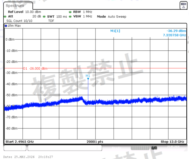
NTNV-BLE_1M-Ant1-2440-2496.5~13000-PASS
