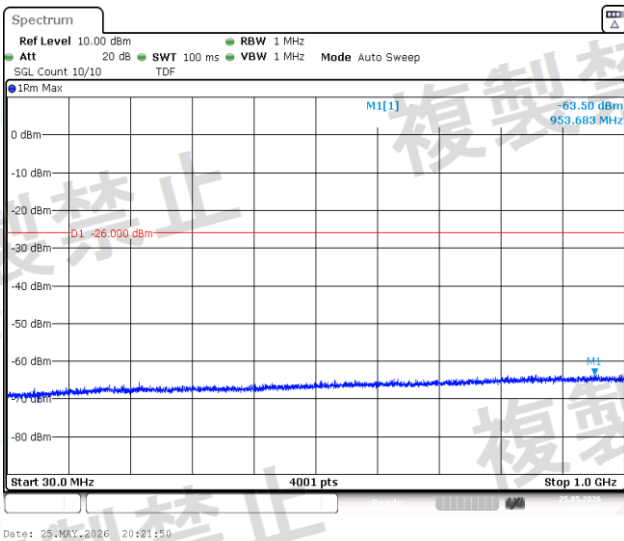
NTNV-BLE_1M-Ant1-2480-30~1000-PASS
