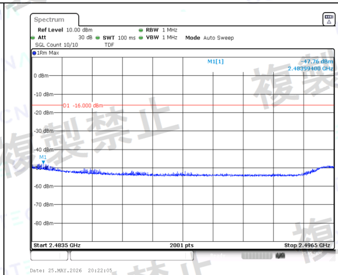
NTNV-BLE_1M-Ant1-2480-2483.5~2496.5-PASS
