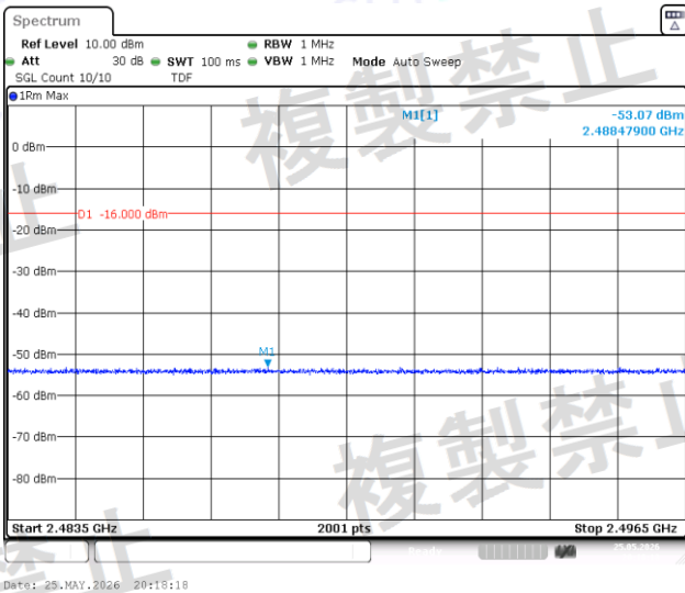
NTNV-BLE_1M-Ant1-2440-2483.5~2496.5-PASS
