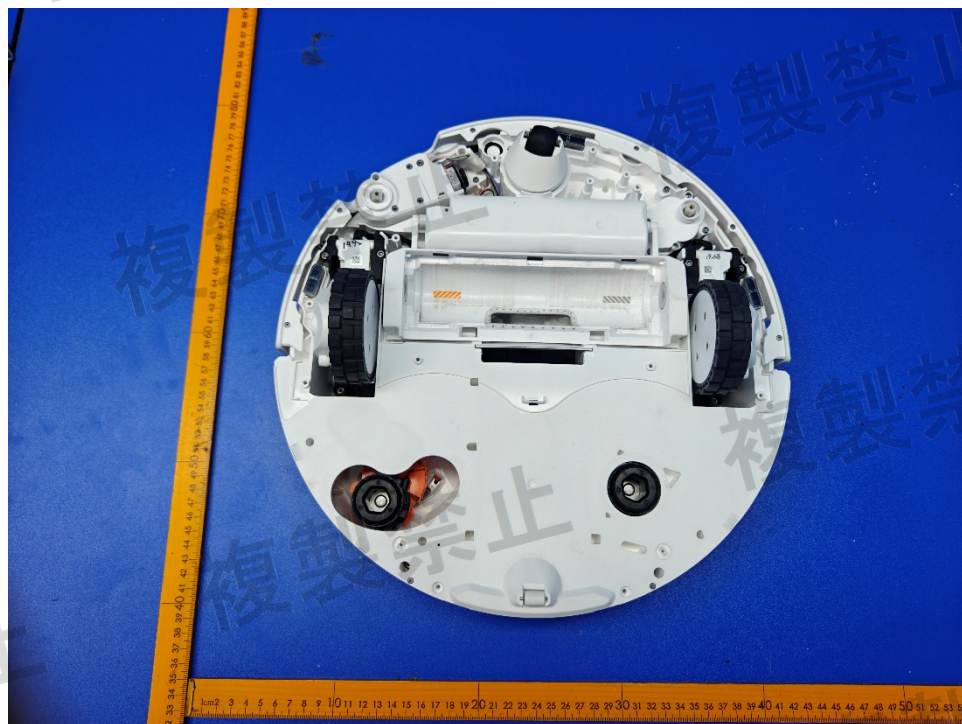
Figure 6. Internal view for model CR8E
