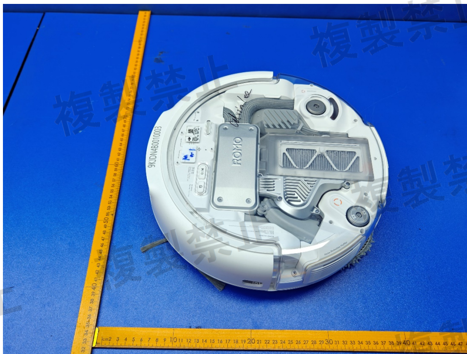
Figure 2. Overall view for model CR8E
