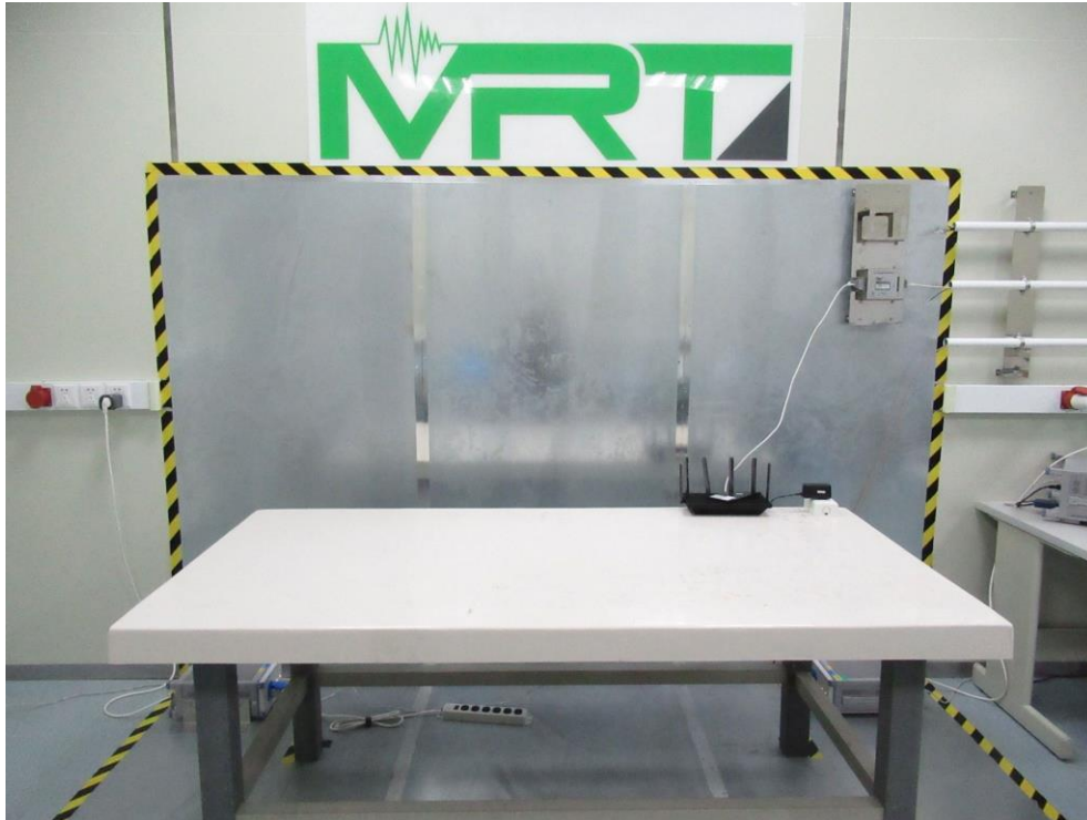
Description: Back View of Conducted Emission Test Setup for Power Port Normal mode
