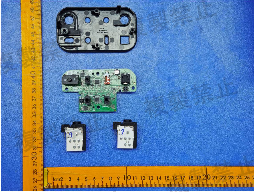
Figure 27: Internal view
