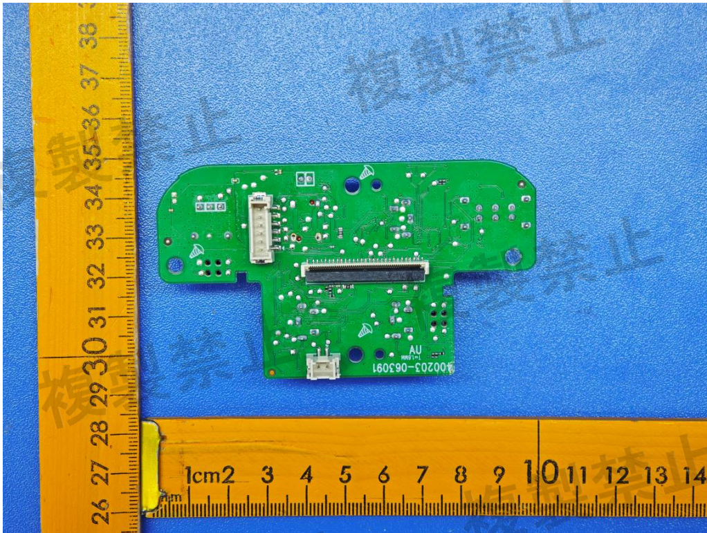
Figure 29: IO board view
