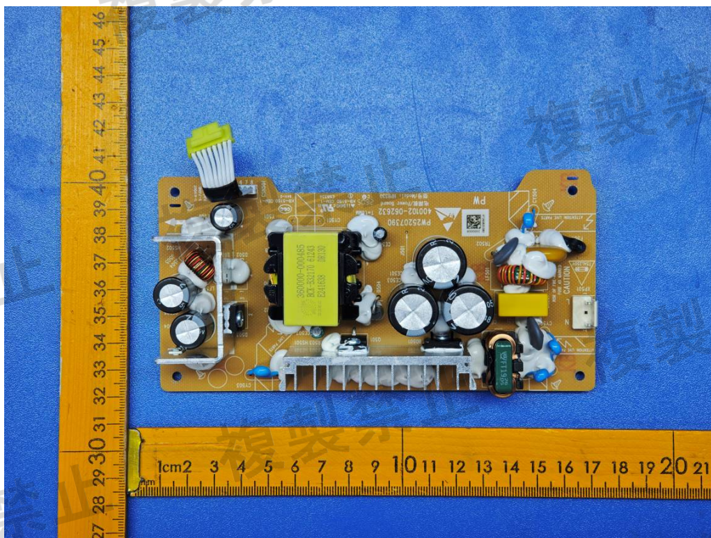
Figure 22: Power board view
