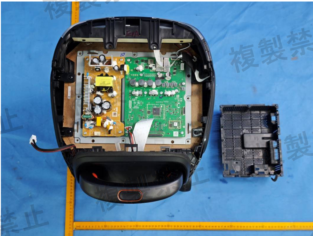
Figure 20: Internal view
