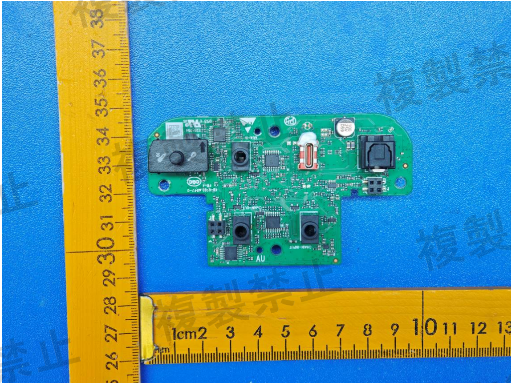
Figure 28: IO board view
