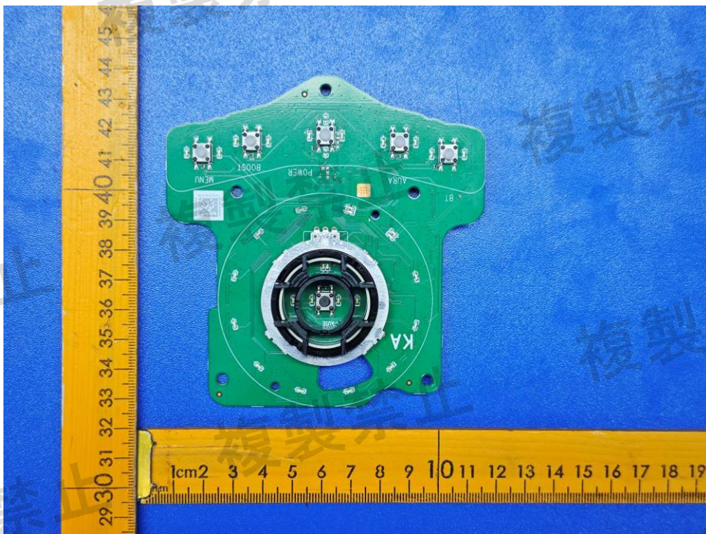
Figure 18: Panel board view
