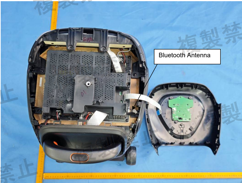
Figure 16: Internal view
