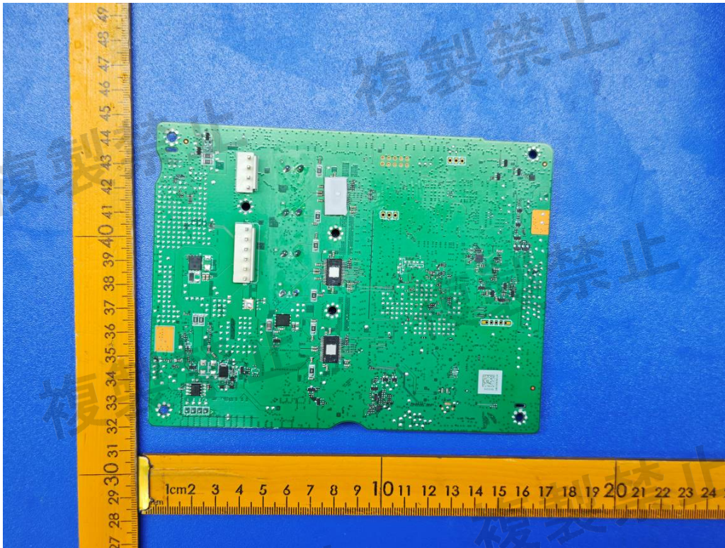
Figure 23: Main board view
