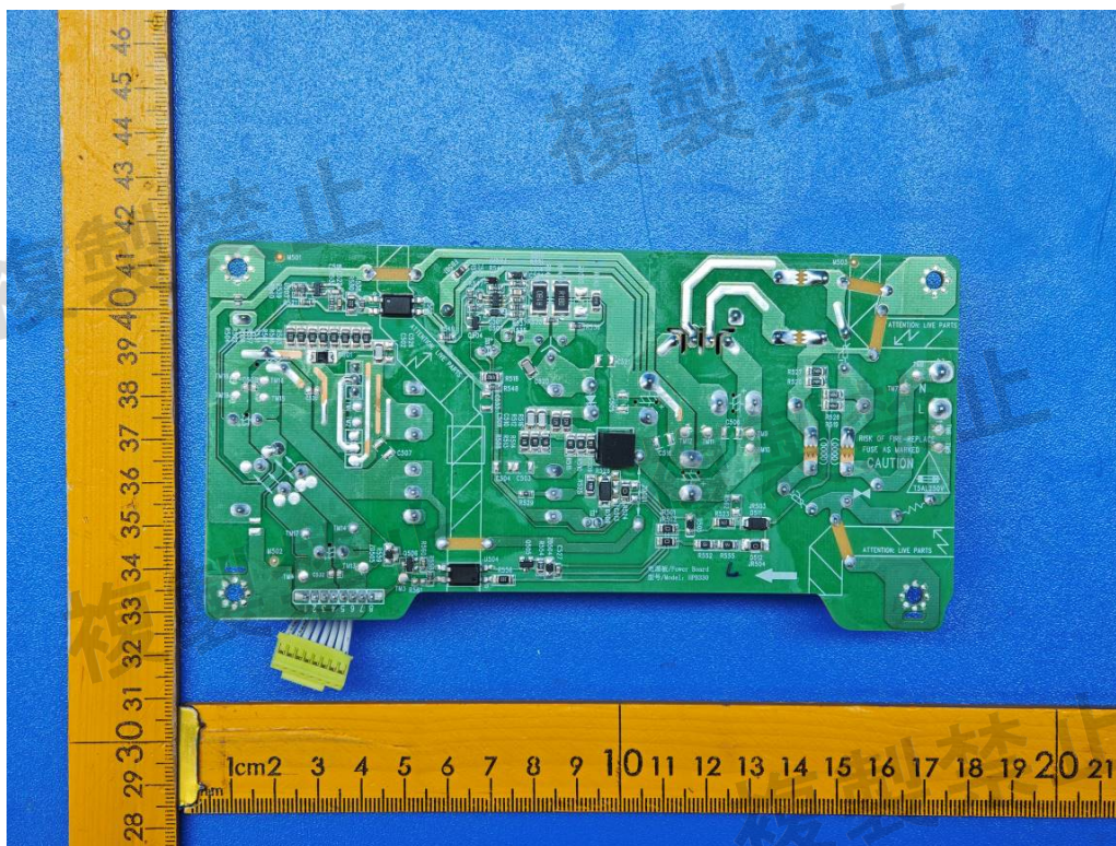
Figure 21: Power board view
