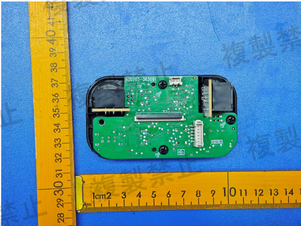
Figure 26: IO port module view
