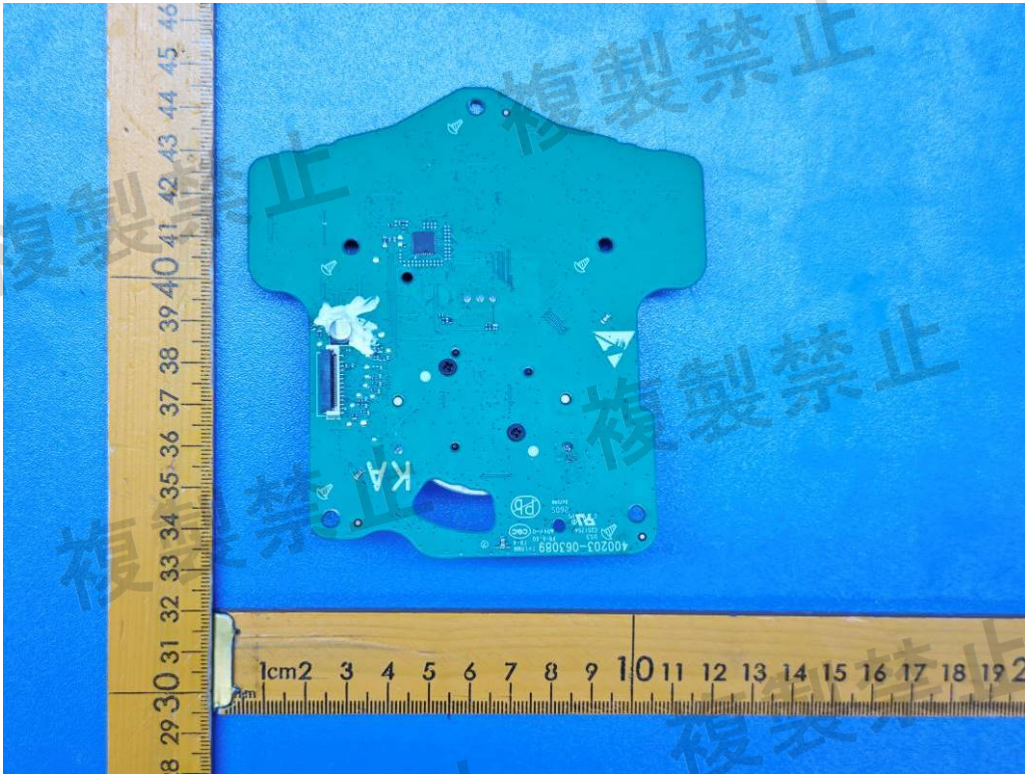
Figure 19: Panel board view
