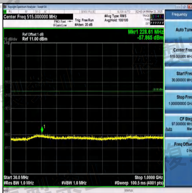
NTNV-11G-Ant1-2472-30~1000-PASS
