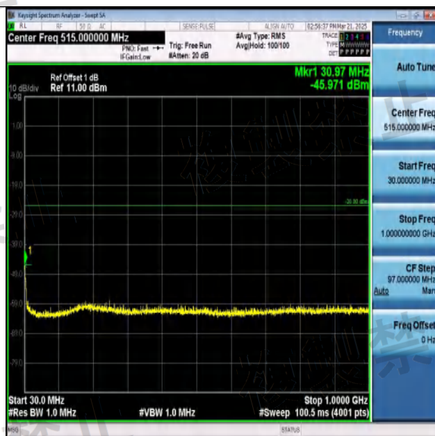
NTNV-11N40SISO-Ant1-2442-30~1000-PASS
