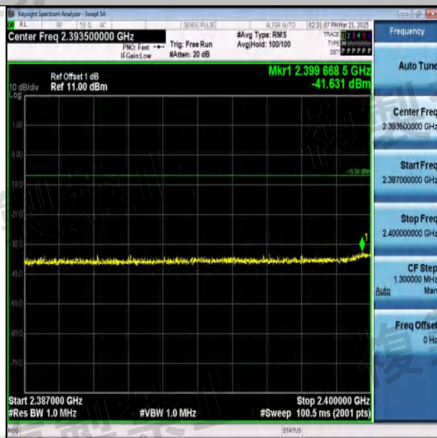
NTNV-11B-Ant1-2442-2387~2400-PASS
