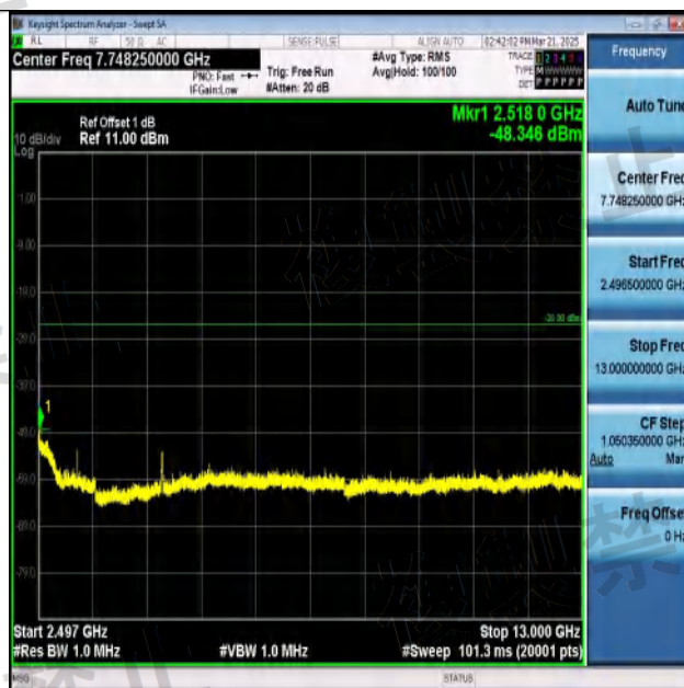
NTNV-11G-Ant1-2442-2496.5~13000-PASS
