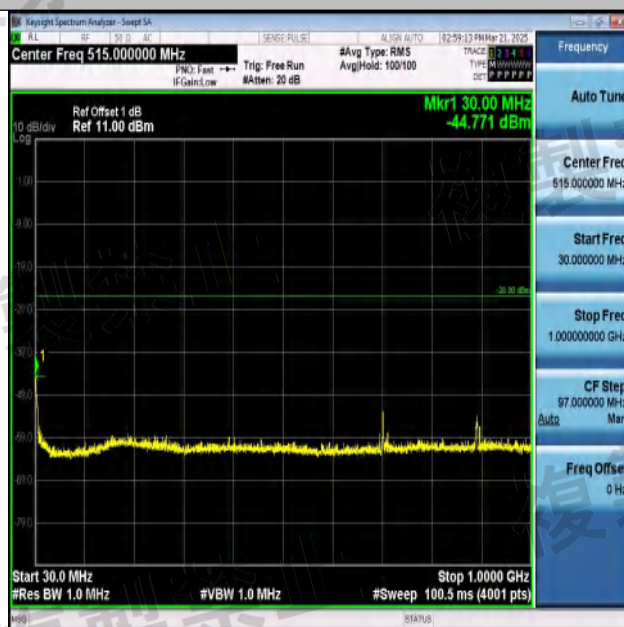
NTNV-11N40SISO-Ant1-2462-30~1000-PASS
