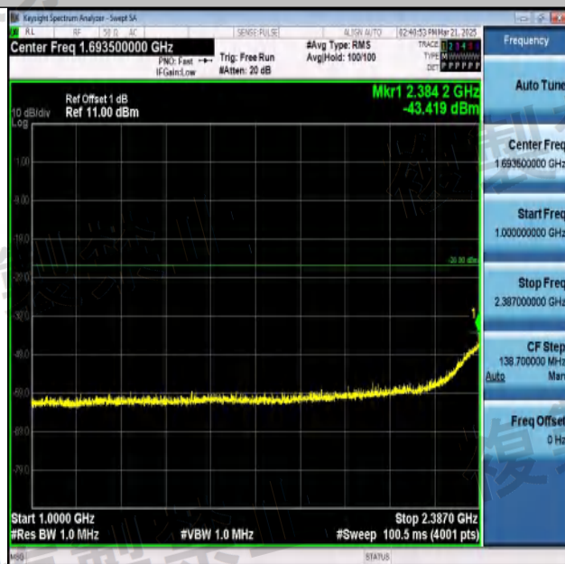
NTNV-11G-Ant1-2442-1000~2387-PASS
