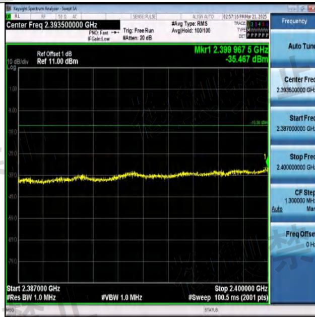
NTNV-11N40SISO-Ant1-2442-2387~2400-PASS
