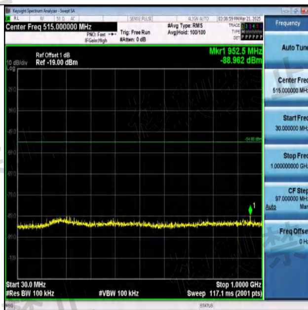
NTNV-11N20SISO-Ant1-2472-30~1000-PASS
