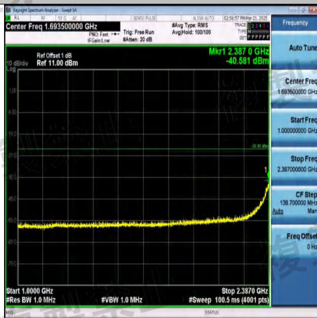
NTNV-11N40SISO-Ant1-2442-1000~2387-PASS
