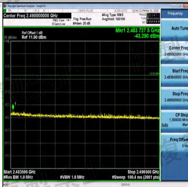
NTNV-11G-Ant1-2442-2483.5~2496.5-PASS
