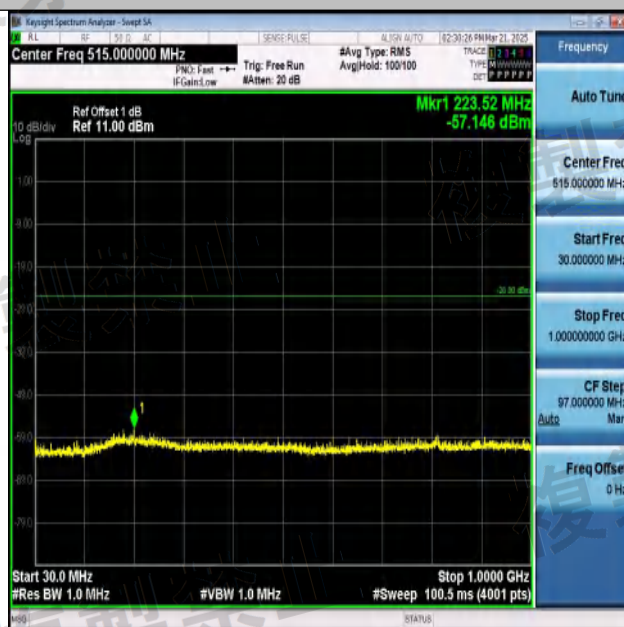
NTNV-11B-Ant1-2442-30~1000-PASS
