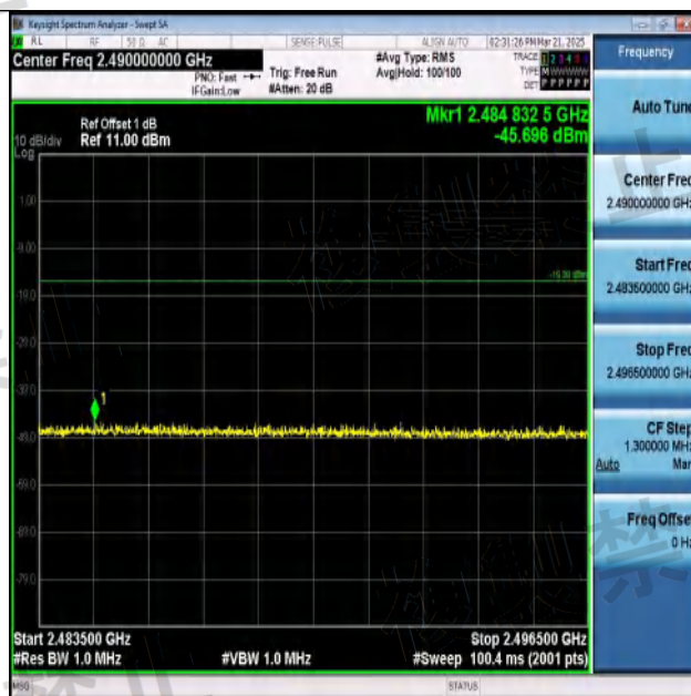
NTNV-11B-Ant1-2442-2483.5~2496.5-PASS
