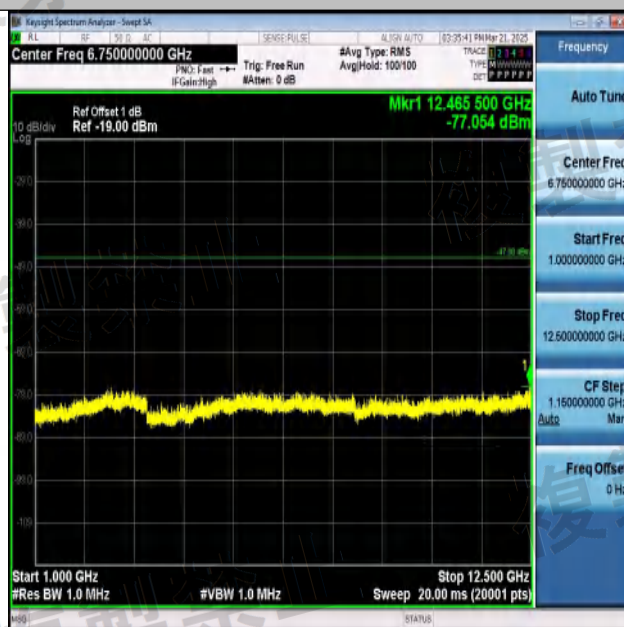
NTNV-11N20SISO-Ant1-2412-1000~12500-PASS
