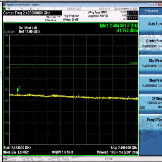
NTNV-11N40SISO-Ant1-2442-2483.5~2496.5-PASS
