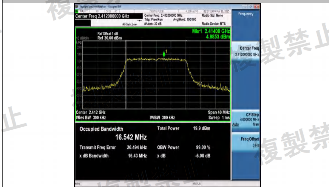
NTNV-11G-Ant1-2412-PASS
