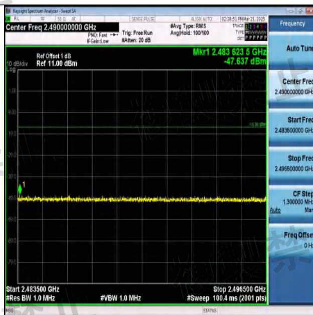
NTNV-11G-Ant1-2412-2483.5~2496.5-PASS
