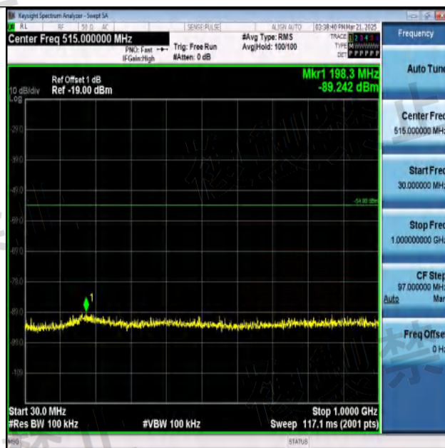
NTNV-11N40SISO-Ant1-2442-30~1000-PASS
