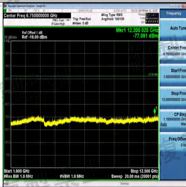
NTNV-11B-Ant1-2472-1000~12500-PASS
