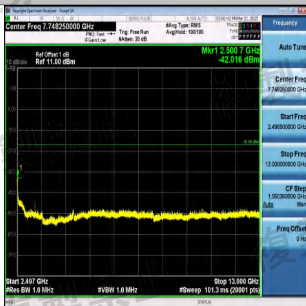
NTNV-11N40SISO-Ant1-2462-2496.5~13000-PASS
