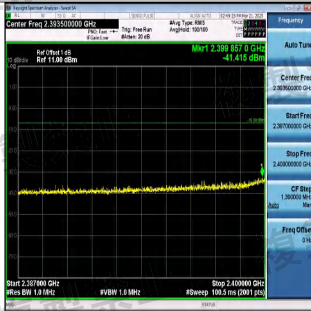
NTNV-11N20SISO-Ant1-2442-2387~2400-PASS
