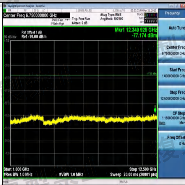
NTNV-11G-Ant1-2442-1000~12500-PASS
