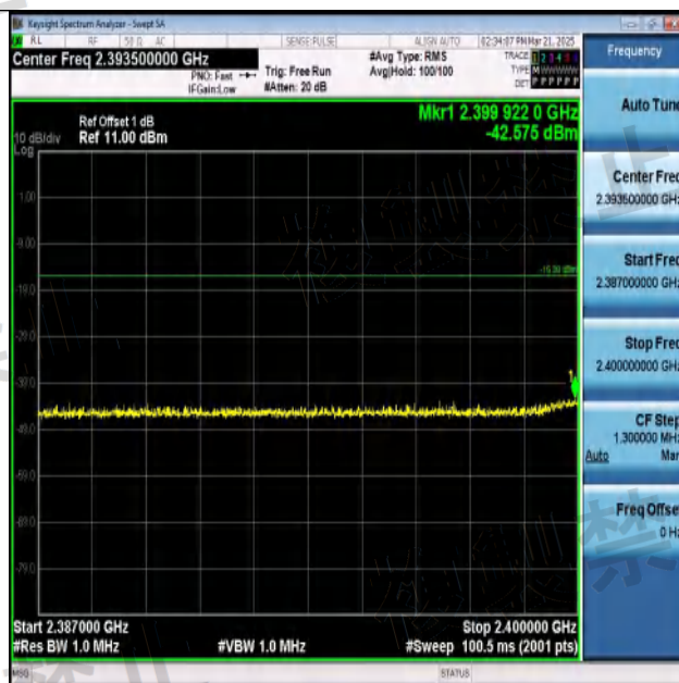
NTNV-11B-Ant1-2472-2387~2400-PASS
