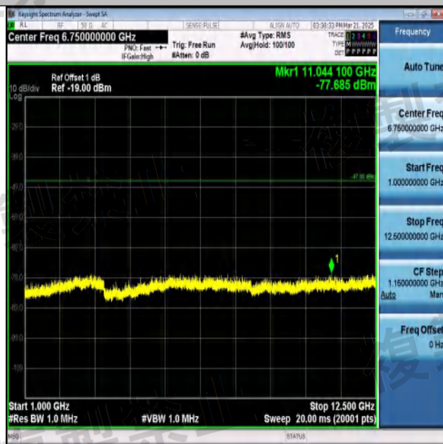
NTNV-11B-Ant1-2442-1000~12500-PASS
