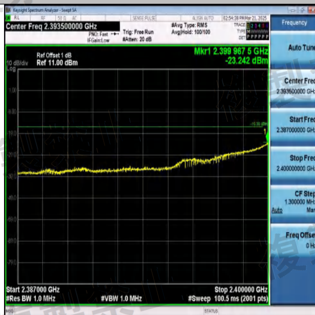
NTNV-11N40SISO-Ant1-2422-2387~2400-PASS
