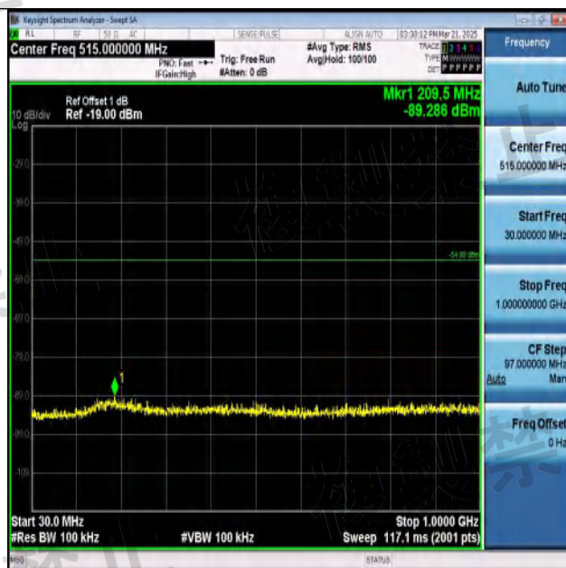
NTNV-11B-Ant1-2442-30~1000-PASS
