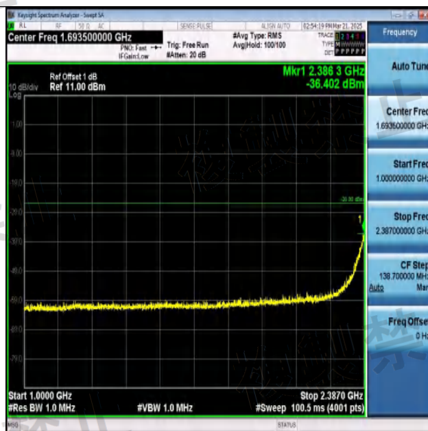
NTNV-11N40SISO-Ant1-2422-1000~2387-PASS
