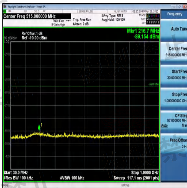
NTNV-11N20SISO-Ant1-2412-30~1000-PASS
