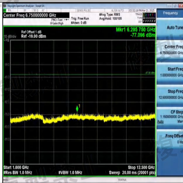
NTNV-11G-Ant1-2412-1000~12500-PASS
