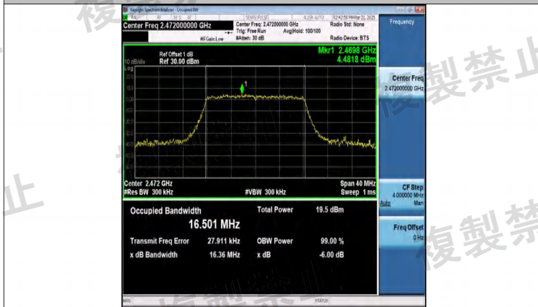
NTNV-11G-Ant1-2472-PASS
