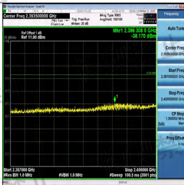
NTNV-11G-Ant1-2442-2387~2400-PASS
