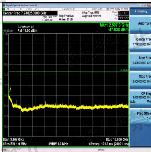
NTNV-11B-Ant1-2412-2496.5~13000-PASS
