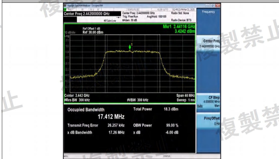
NTNV-11N20SISO-Ant1-2442-PASS
