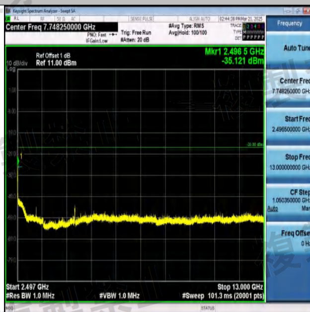
NTNV-11G-Ant1-2472-2496.5~13000-PASS
