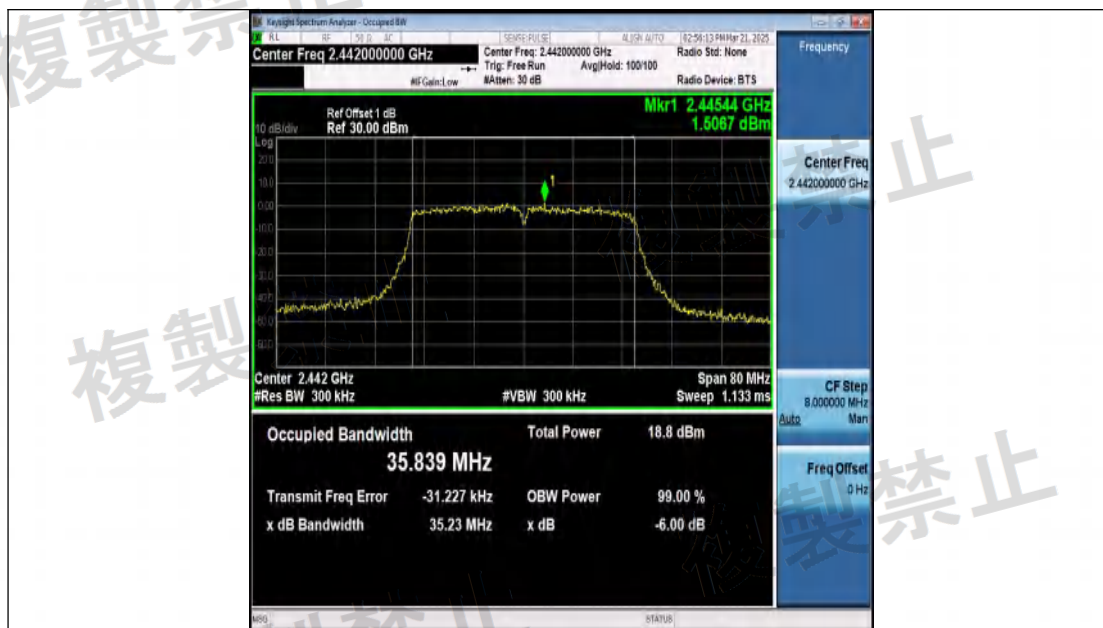
NTNV-11N40SISO-Ant1-2442-PASS
