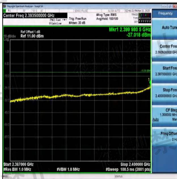
NTNV-11N20SISO-Ant1-2412-2387~2400-PASS
