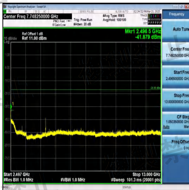
NTNV-11B-Ant1-2472-2496.5~13000-PASS
