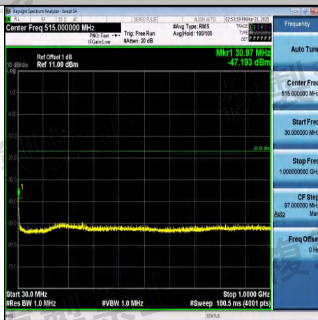
NTNV-11N40SISO-Ant1-2422-30~1000-PASS
