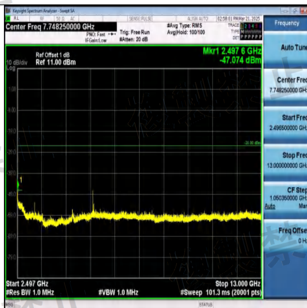
NTNV-11N40SISO-Ant1-2442-2496.5~13000-PASS
