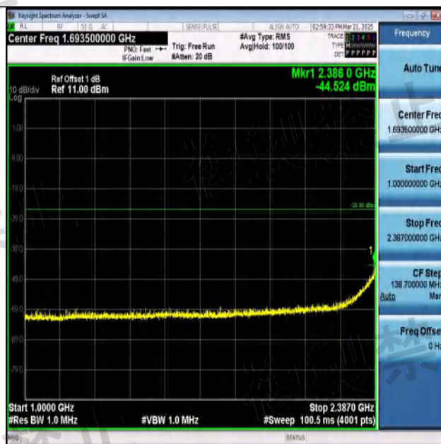
NTNV-11N40SISO-Ant1-2462-1000~2387-PASS
