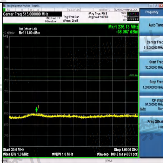
NTNV-11G-Ant1-2442-30~1000-PASS
