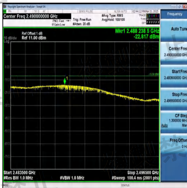
NTNV-11G-Ant1-2472-2483.5~2496.5-PASS
