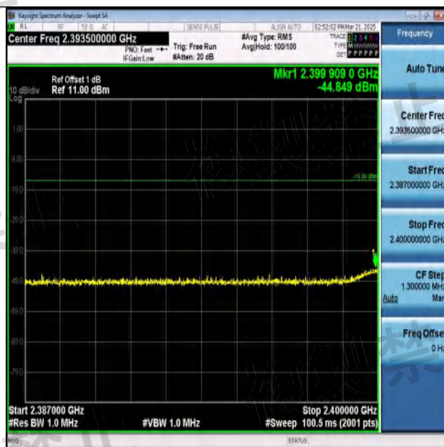
NTNV-11N20SISO-Ant1-2472-2387~2400-PASS
