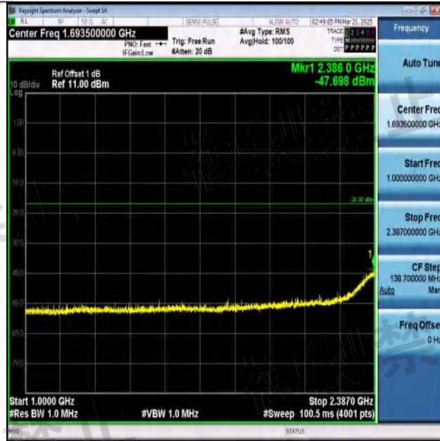
NTNV-11N20SISO-Ant1-2442-1000~2387-PASS
