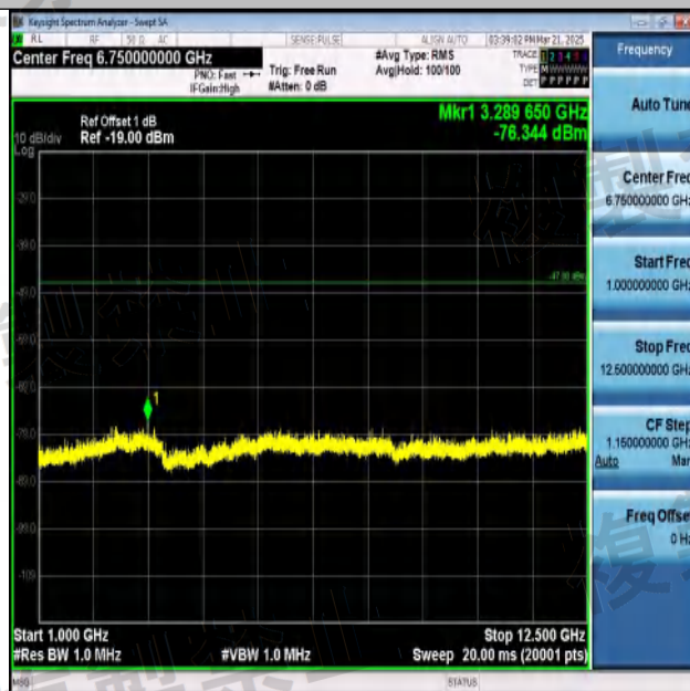
NTNV-11N40SISO-Ant1-2442-1000~12500-PASS
