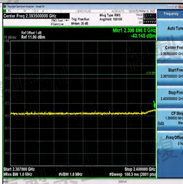
NTNV-11G-Ant1-2472-2387~2400-PASS
