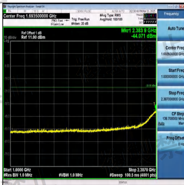
NTNV-11B-Ant1-2442-1000~2387-PASS
