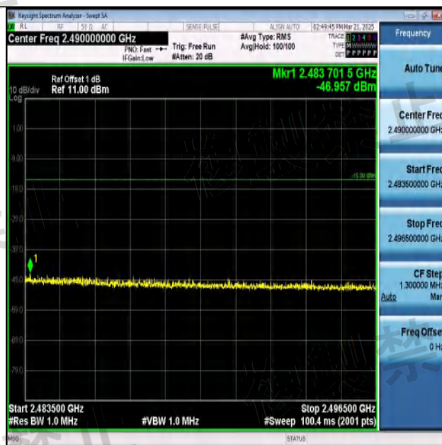
NTNV-11N20SISO-Ant1-2442-2483.5~2496.5-PASS
