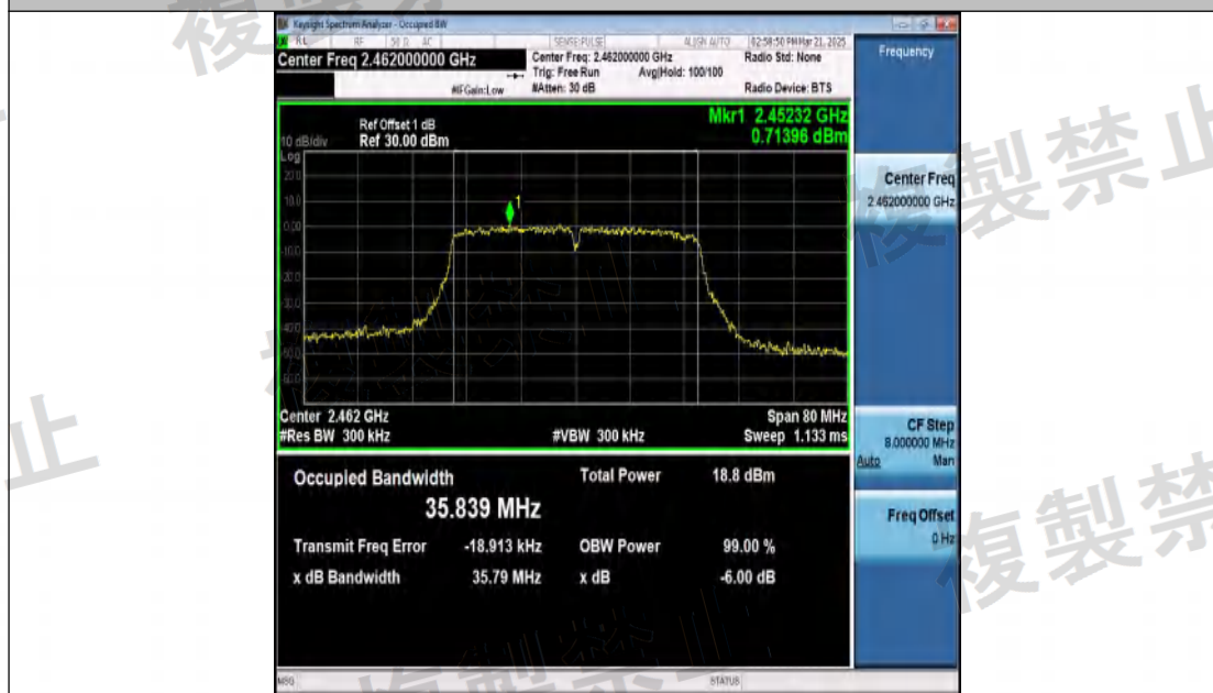
NTNV-11N40SISO-Ant1-2462-PASS
