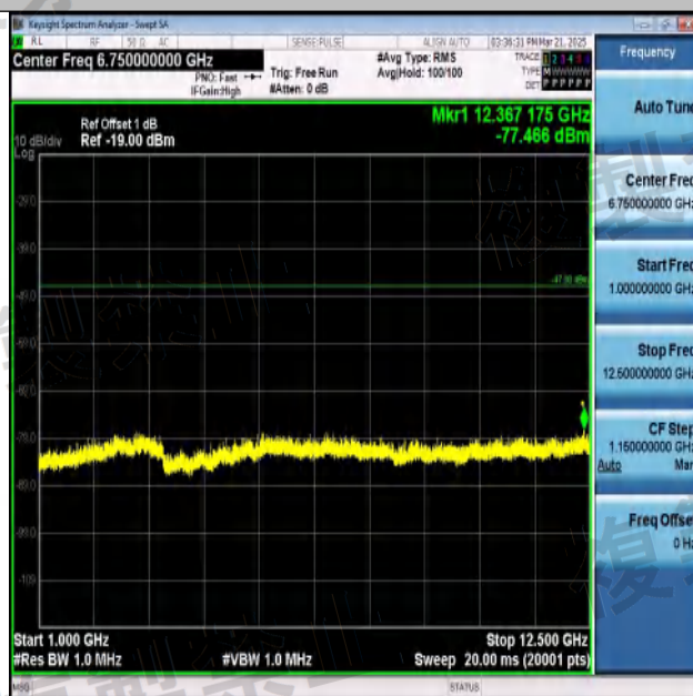
NTNV-11N20SISO-Ant1-2442-1000~12500-PASS
