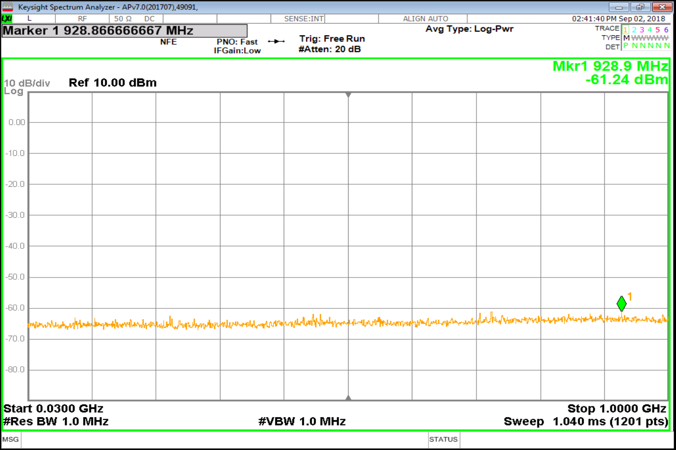
Tx3_SpuriousM_Nom
