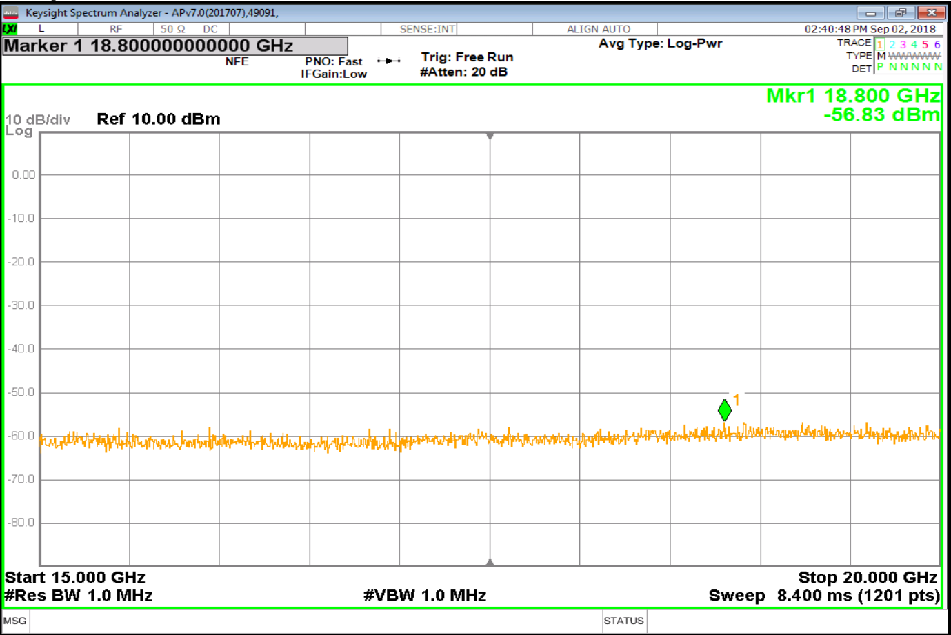
Tx3_SpuriousG4_Nom
