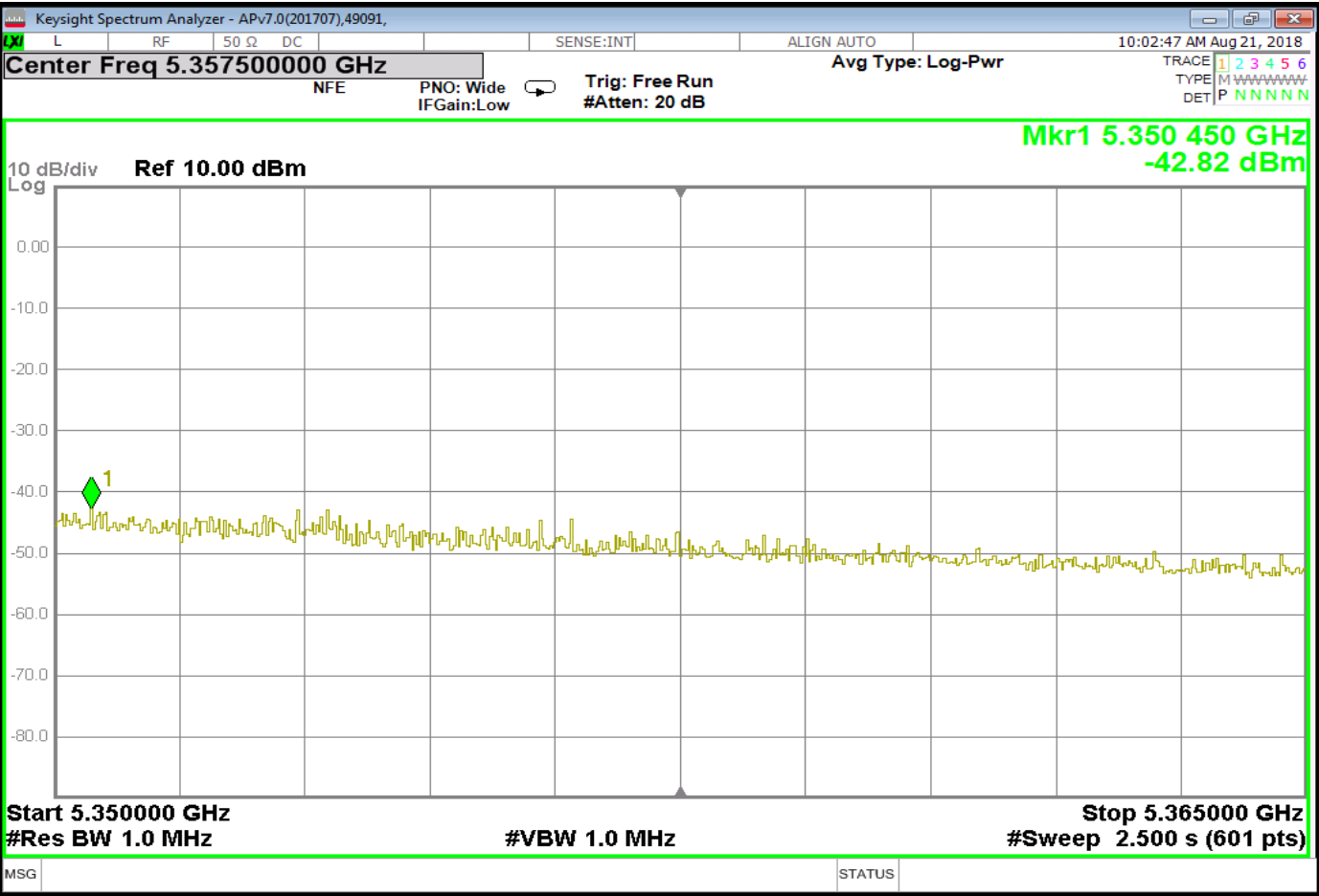
Tx1_Leak5_Nom
