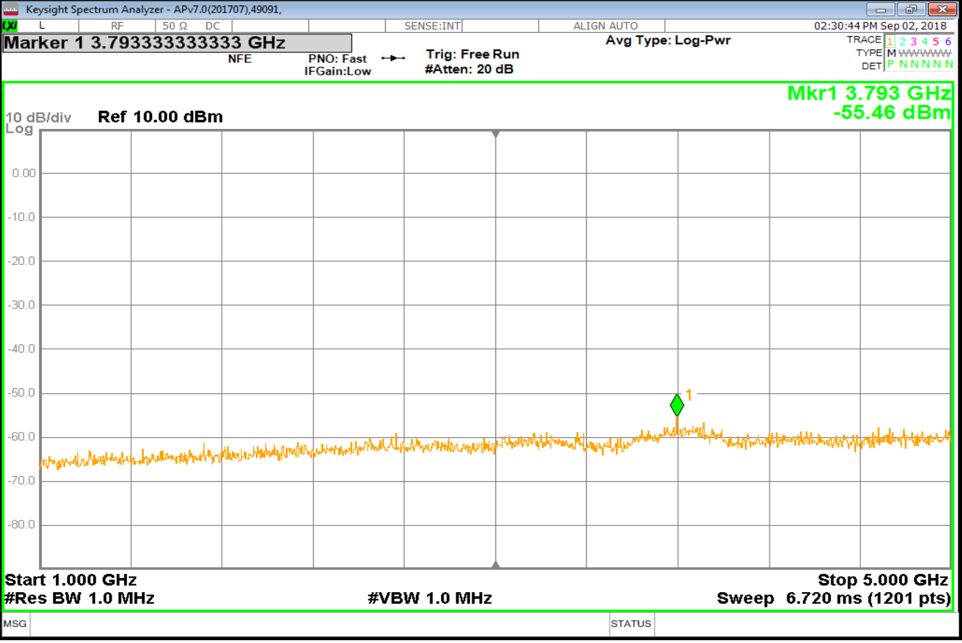
Tx1_SpuriousG1_Nom
