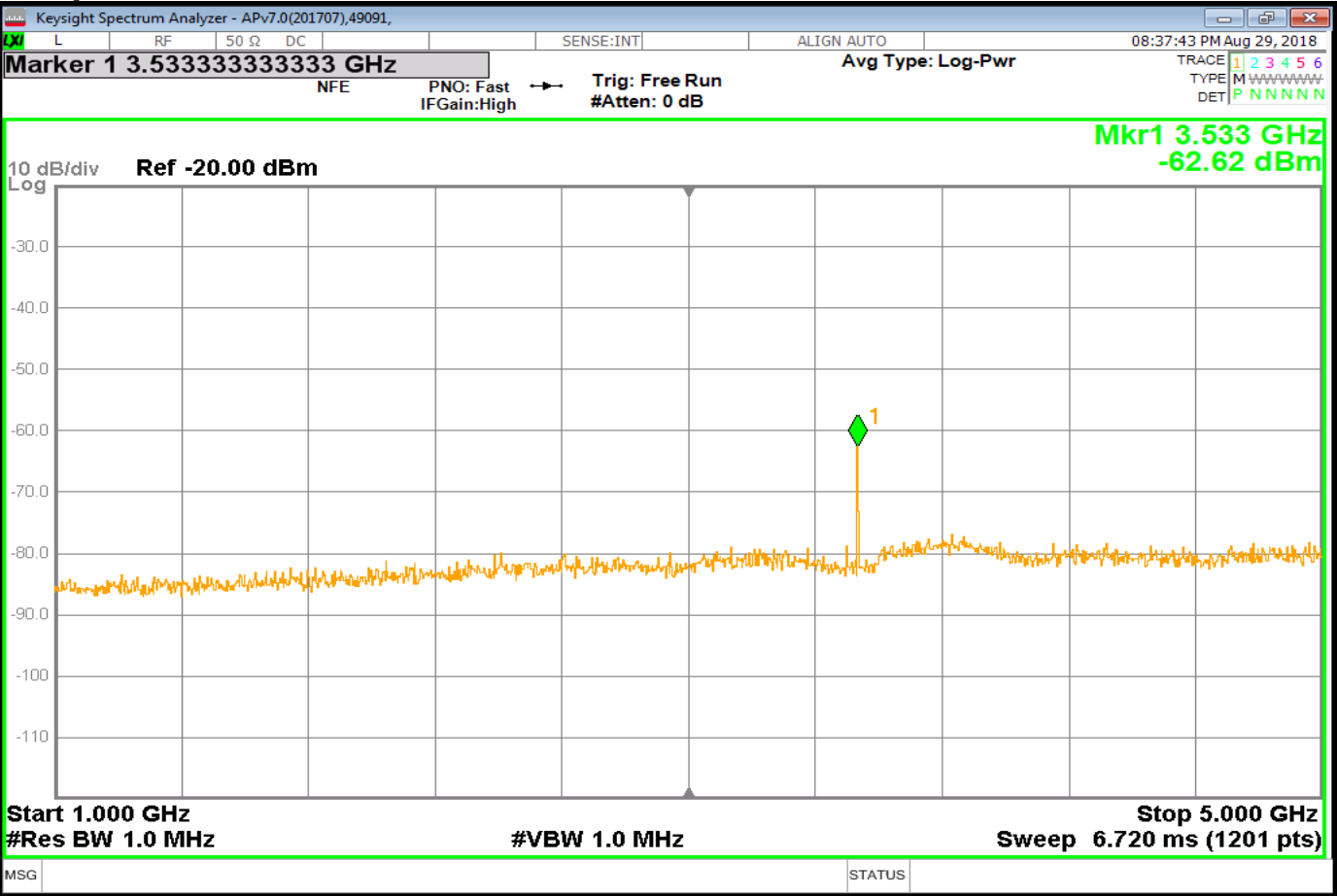
Rx1_SpuriousG1_Nom
