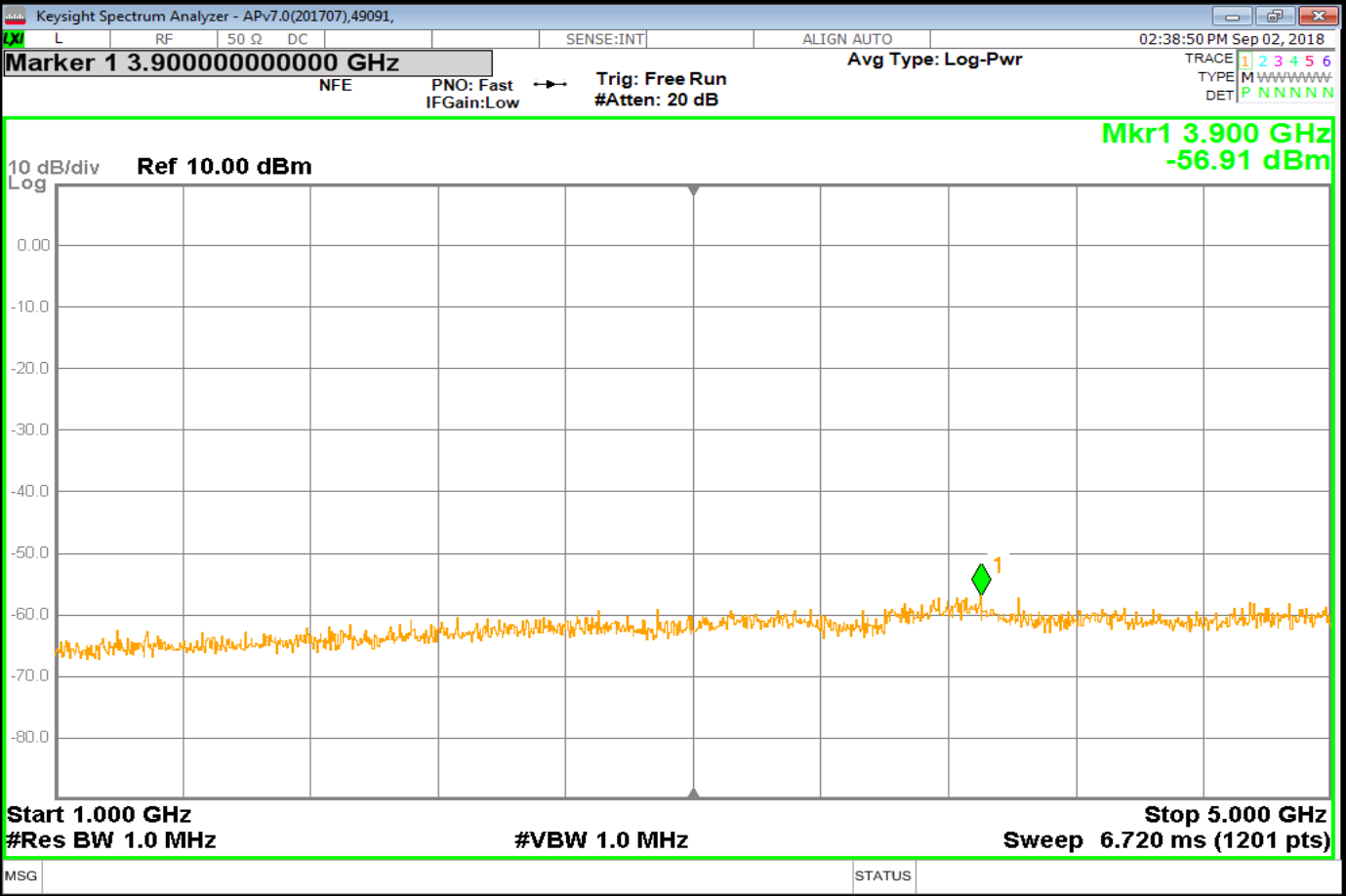
Tx3_SpuriousG1_Nom
