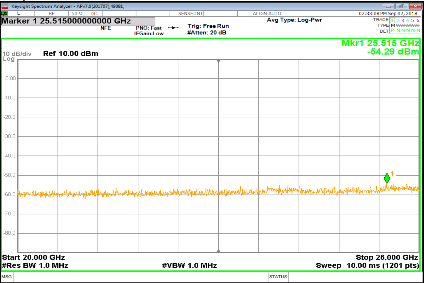
Tx1_SpuriousG5_Nom
