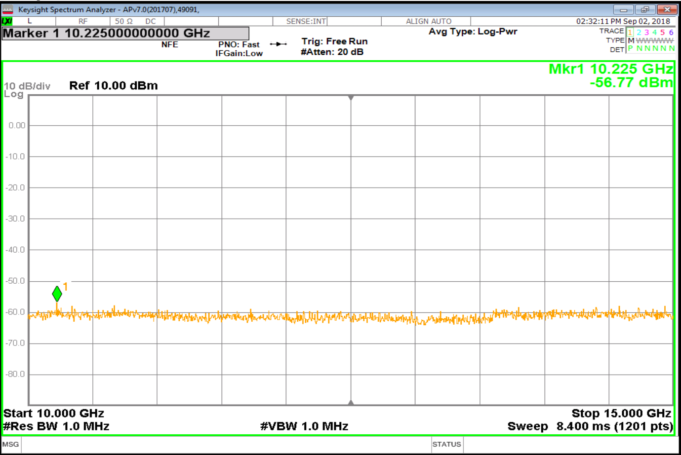
Tx1_SpuriousG3_Nom
