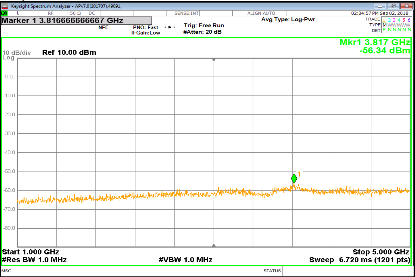
Tx2_SpuriousG1_Nom
