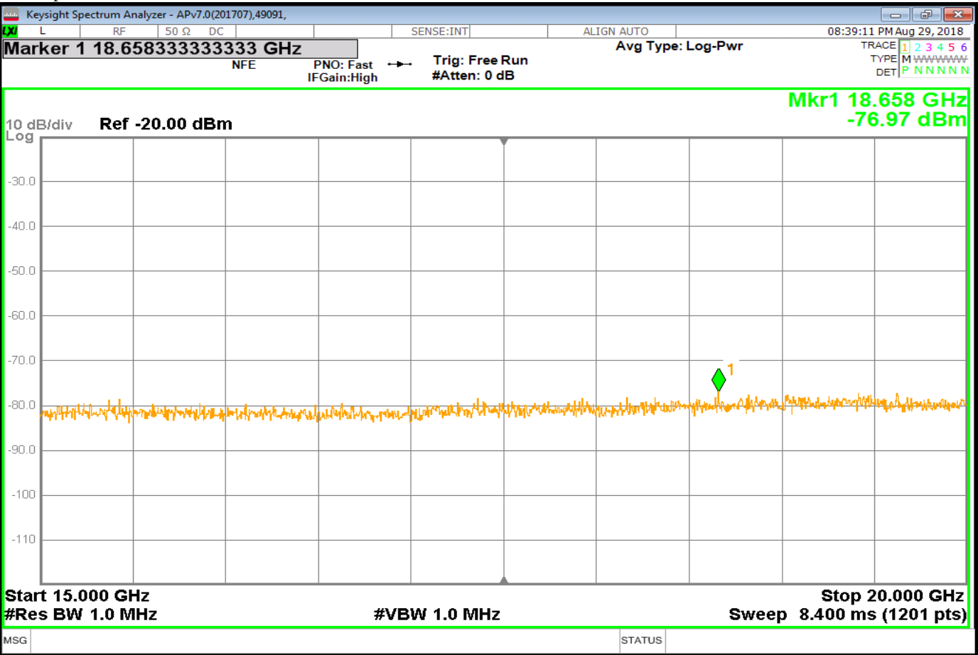
Rx1_SpuriousG4_Nom
