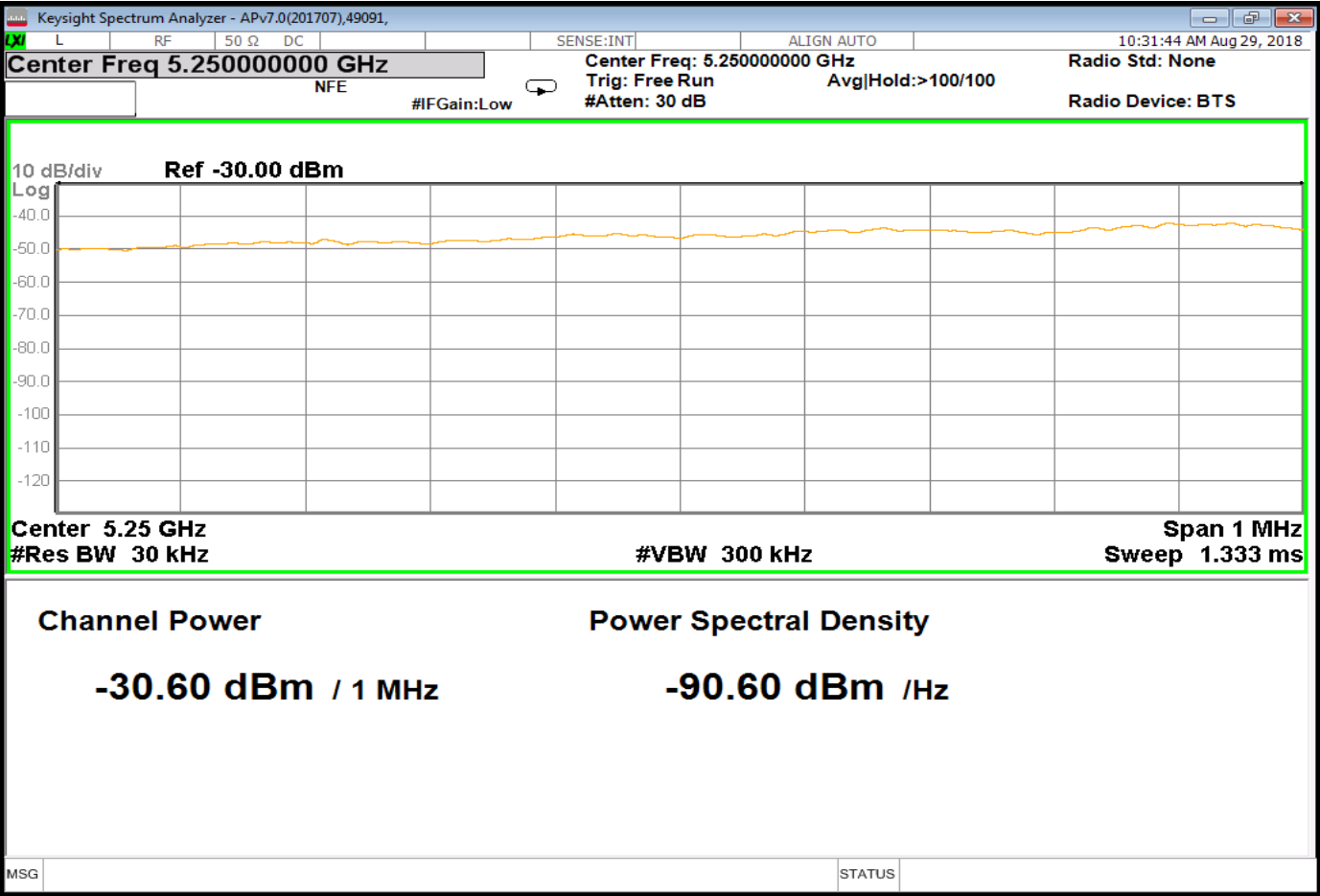
Tx1_Leak4Zoom_Nom
