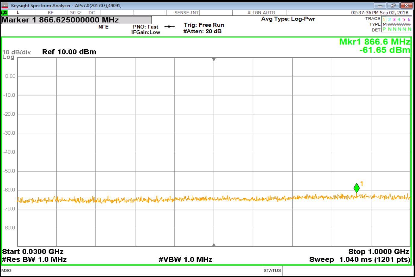
Tx2_SpuriousM_Nom
