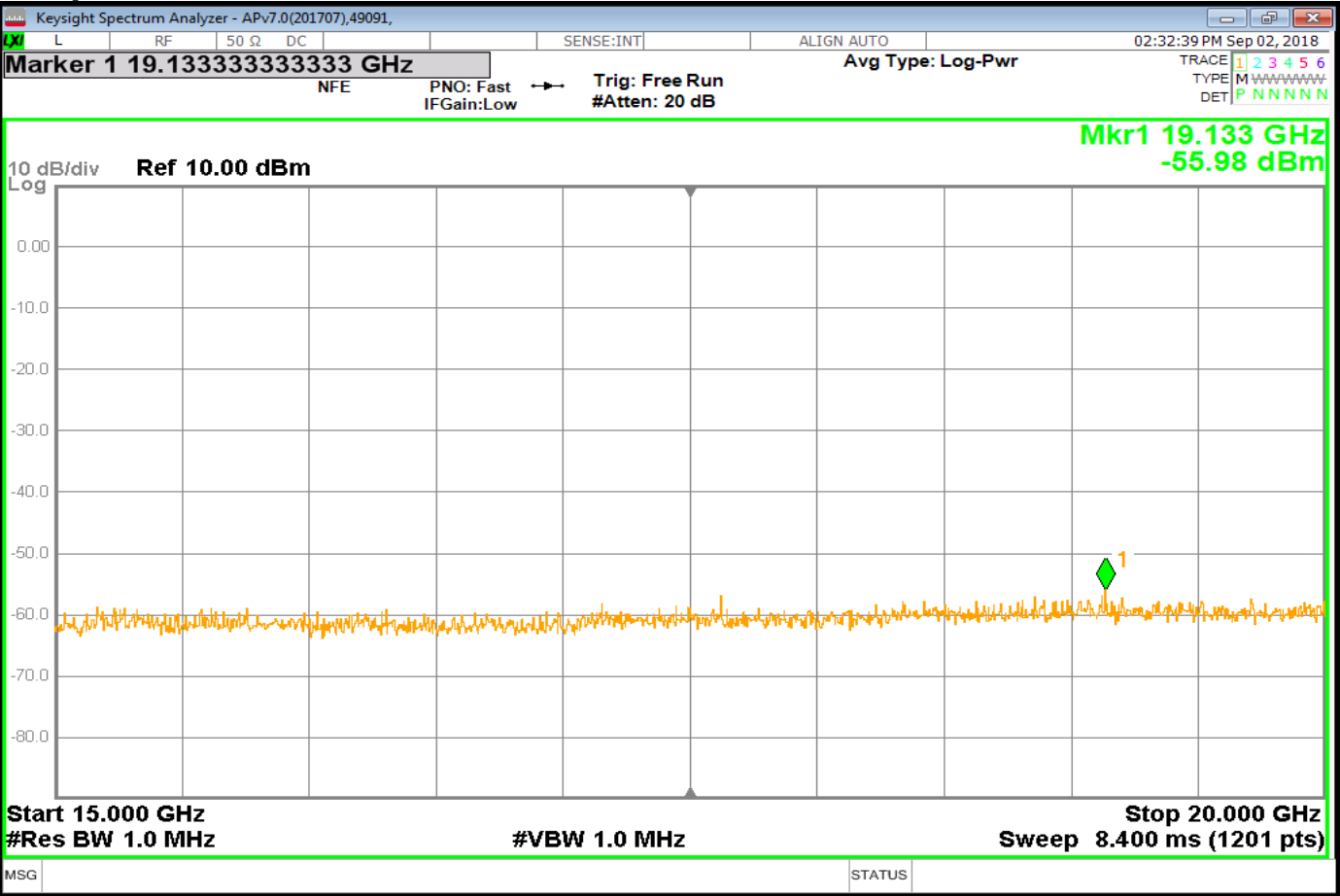
Tx1_SpuriousG4_Nom
