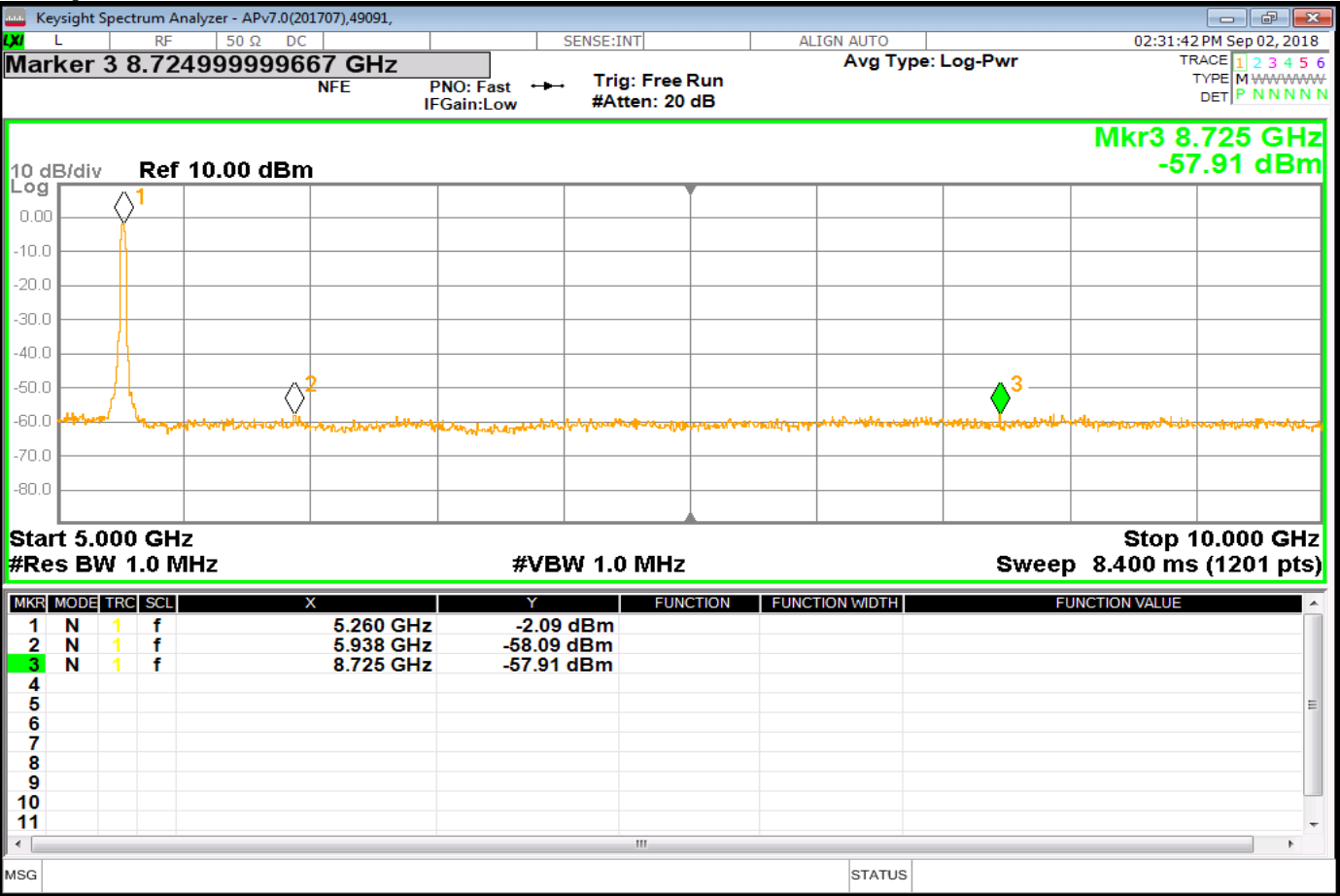
Tx1_SpuriousG2_Nom
