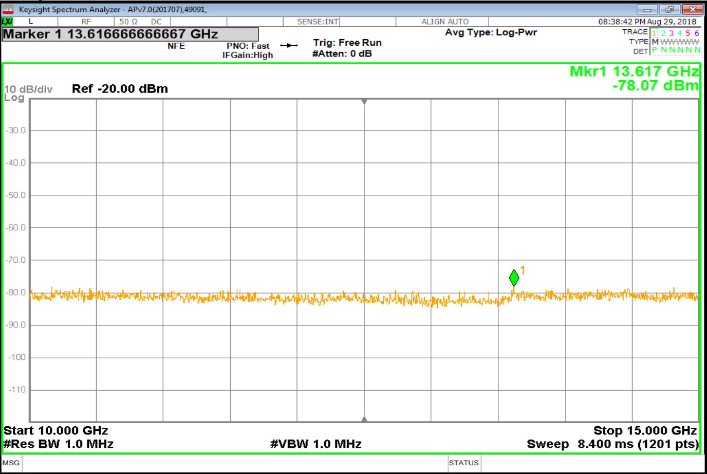
Rx1_SpuriousG3_Nom
