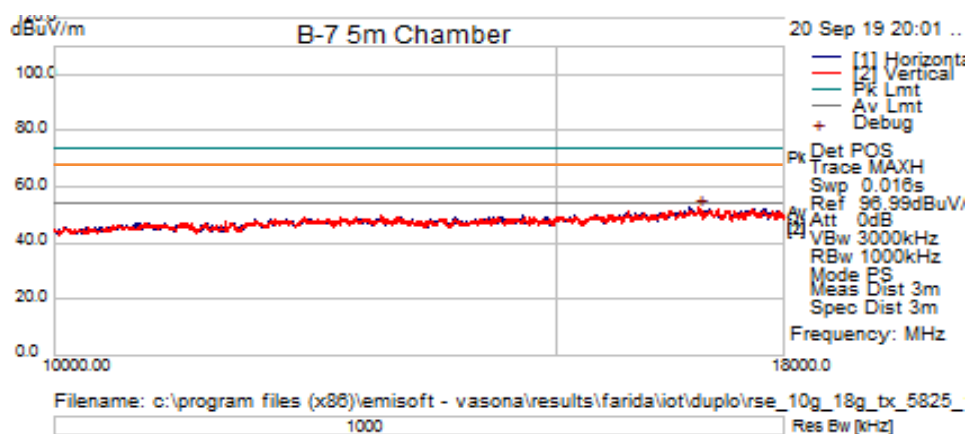
Title: TX Spurious Emissions from 10GHz-18GHz – Ch165 (5825 MHz)
