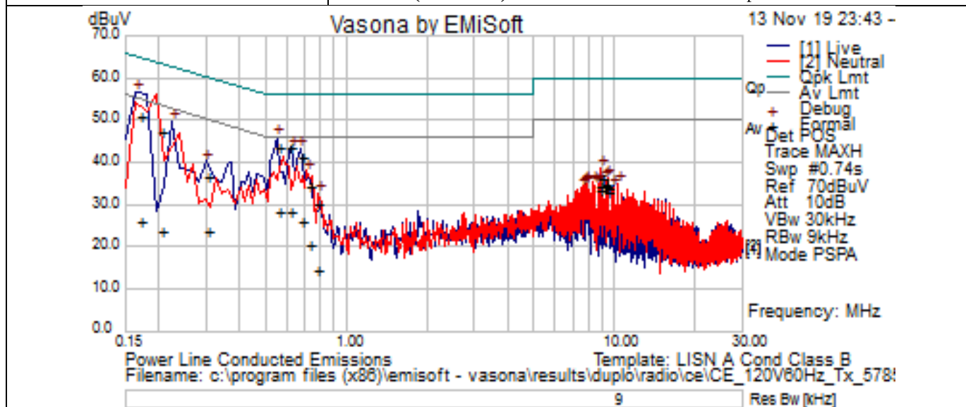
AC Conducted Emissions Test Result Tables for 802.11a / TX Ch157
