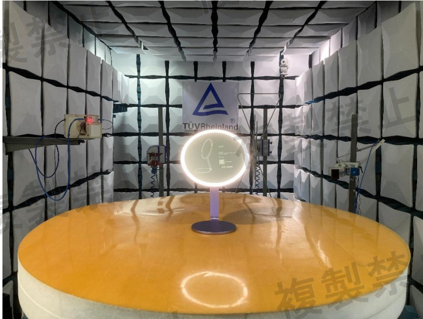
Photograph 1: Set-up for Radio Spectrum Spurious Testing
