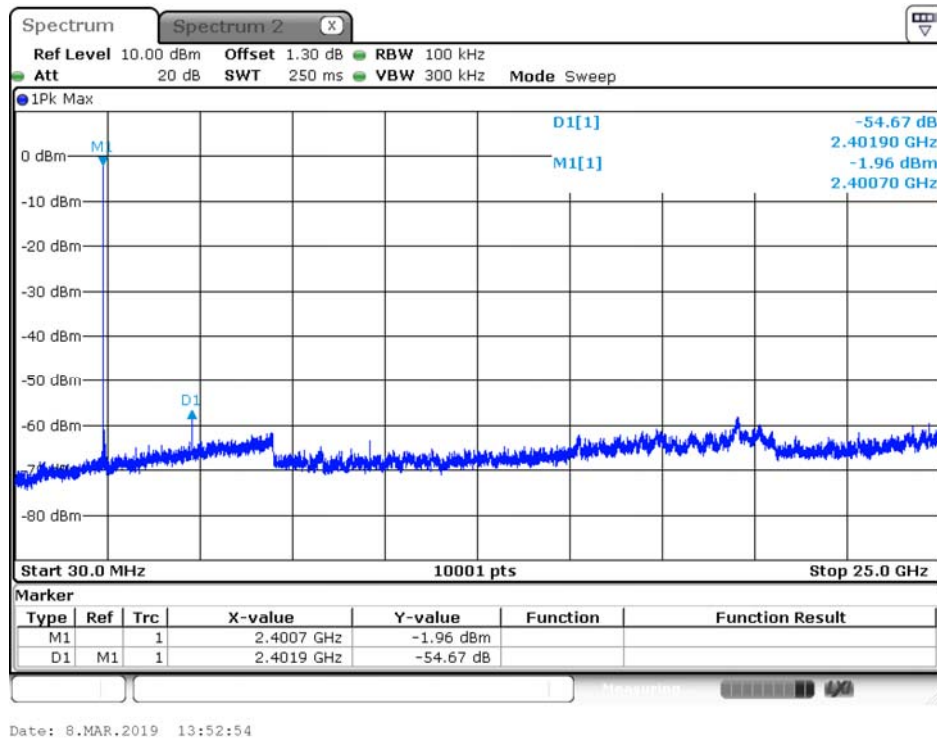
Channel 00 (30MHz-25GHz)
