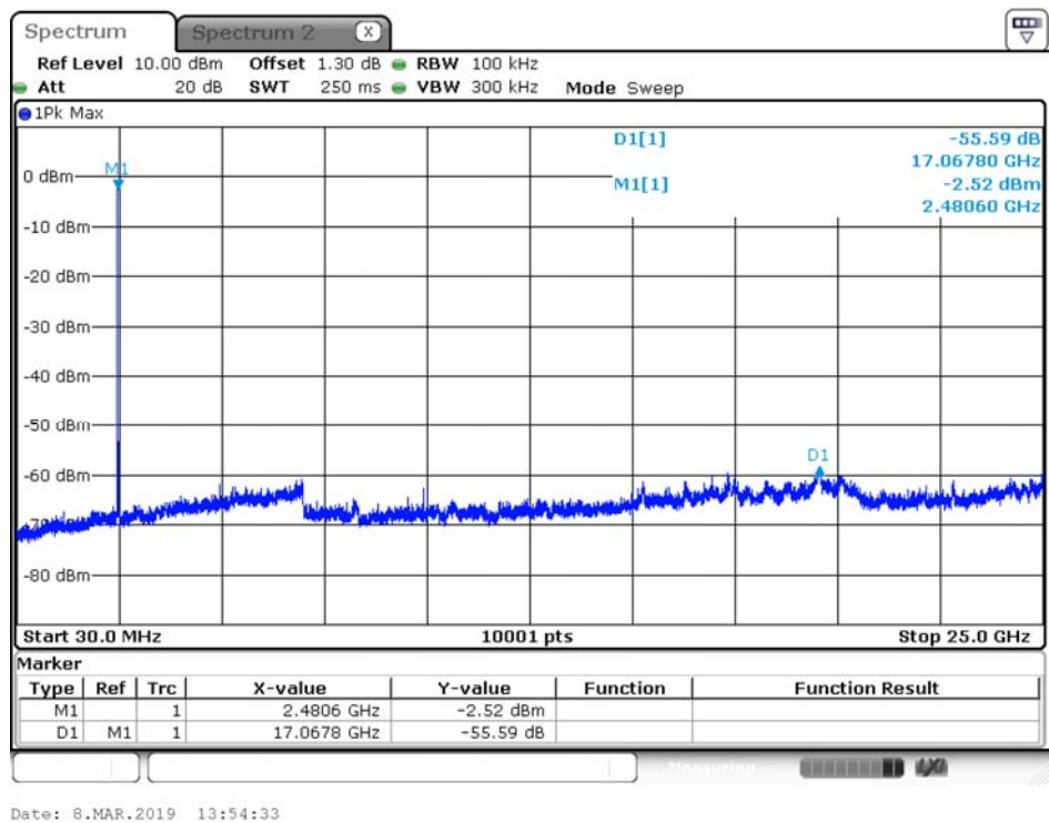
Channel 39 (30MHz-25GHz)
