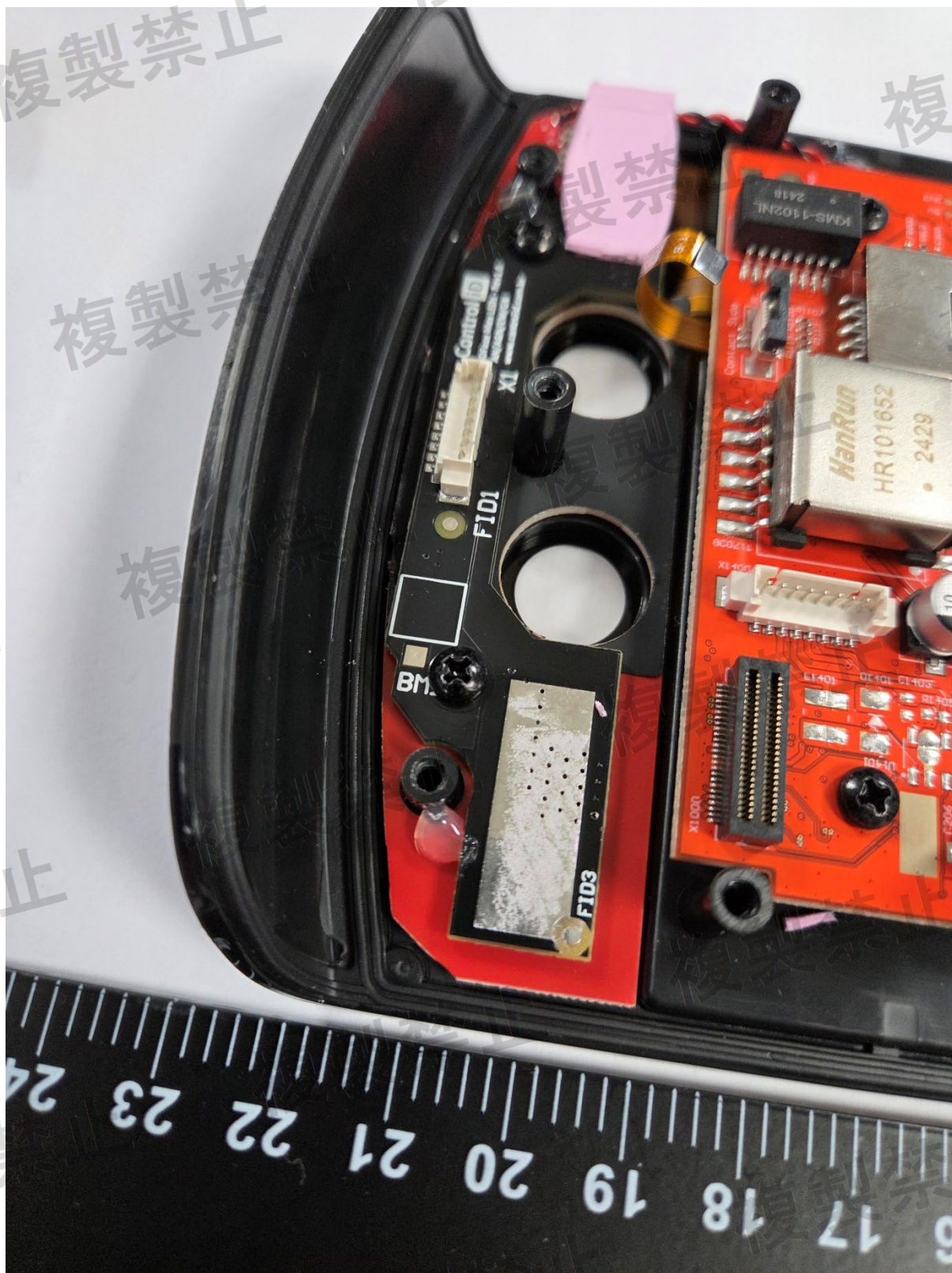
HF Antenna position
