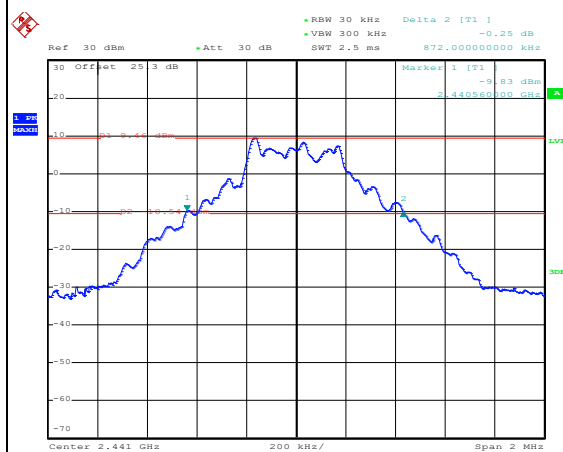
20 dB Bandwidth Plot on Channel 39
