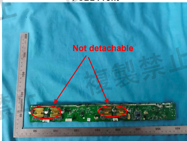
PCB3 Front
