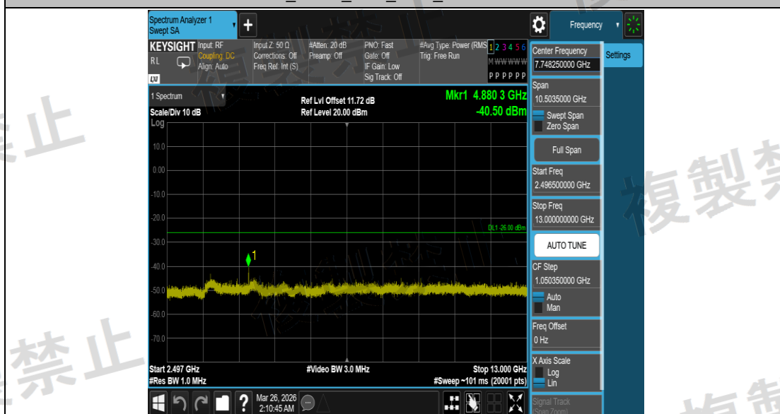
NTNV_GFSK_Ant1_2440_2496.5~13000
