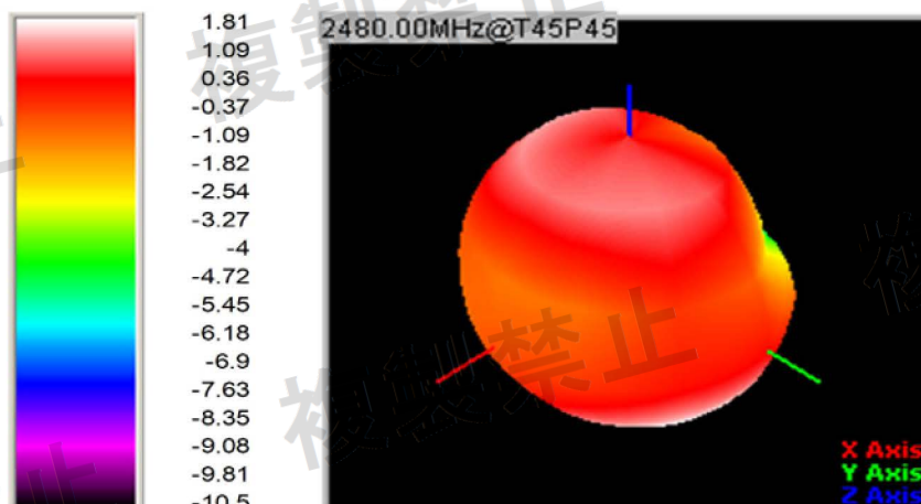
© 3D Gain Pattern (2480 MHz)
