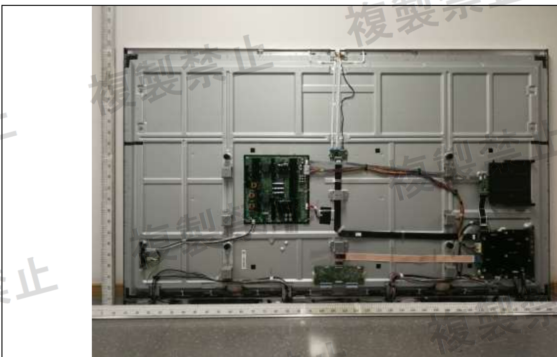
Details of: Internal view 5 (with construction B of power supply board and FFC wire 1)
