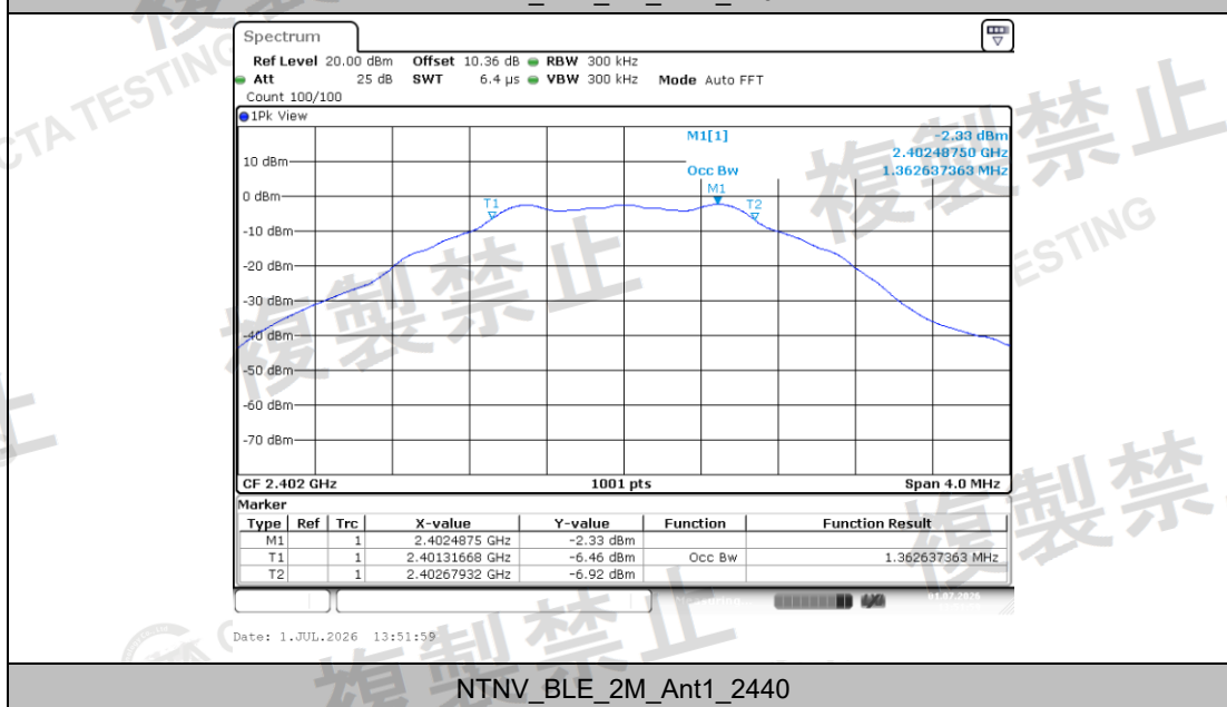
NTNV_BLE_2M_Ant1_2402
