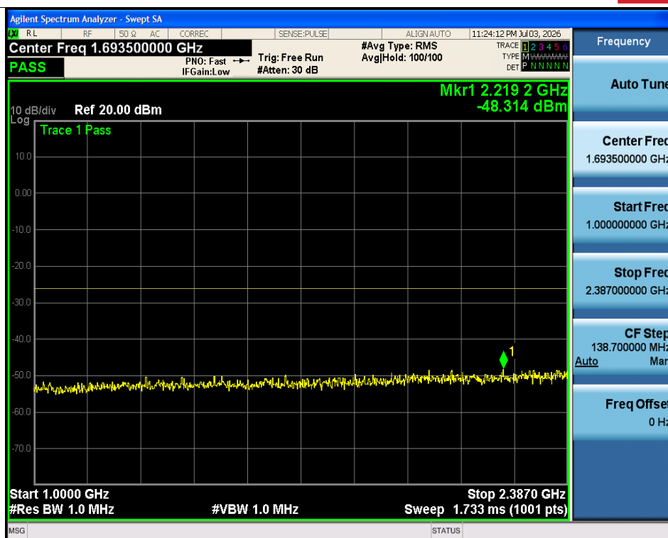
Tx. Spurious NVNT 2480MHz Ant1 @ 1000MHz-2387MHz
