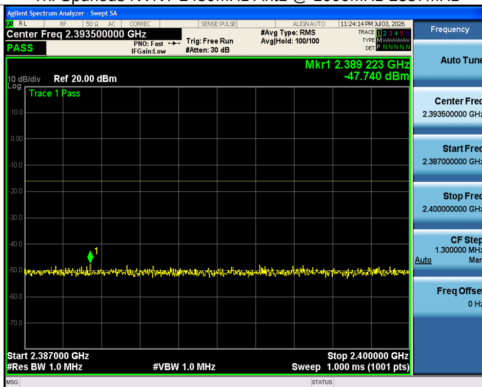
Tx. Spurious NVNT 2480MHz Ant1 @ 2387MHz-2400MHz
