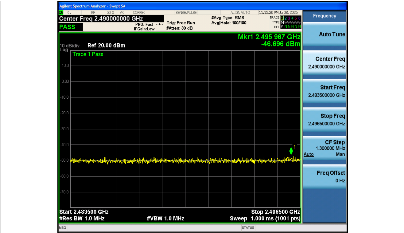
Tx. Spurious NVNT 2402MHz Ant1 @ 2483.5MHz-2496.5MHz
