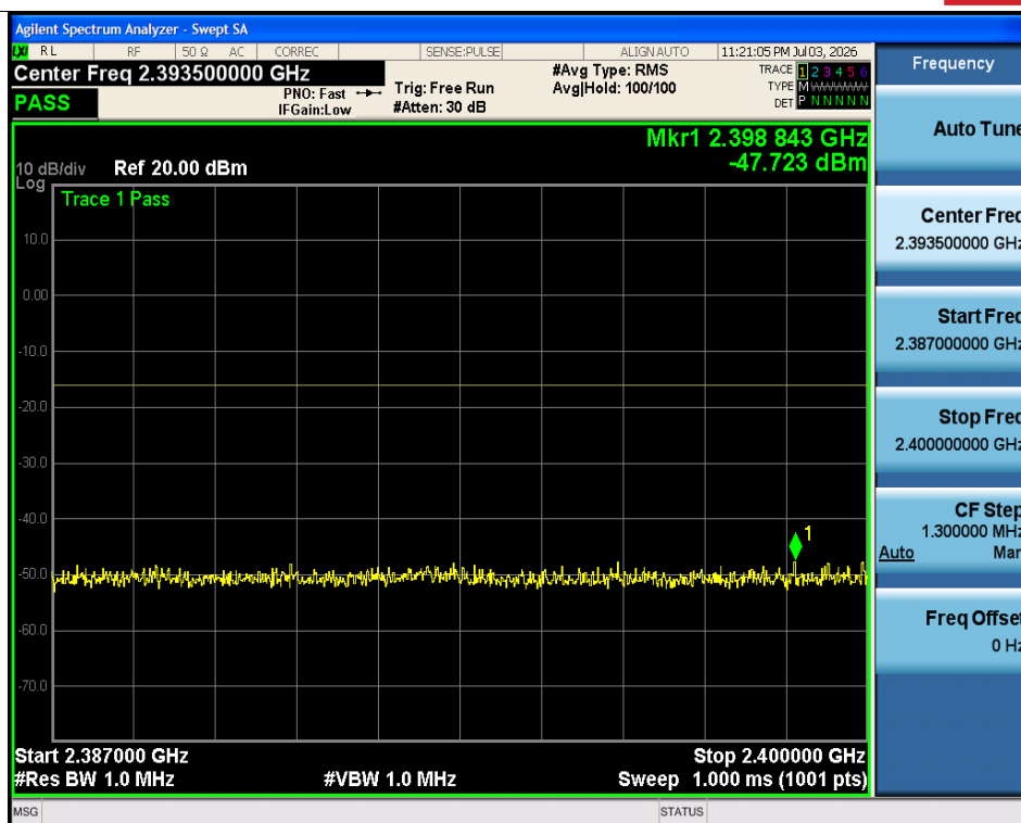
Tx. Spurious NVNT 2441MHz Ant1 @ 2387MHz-2400MHz
