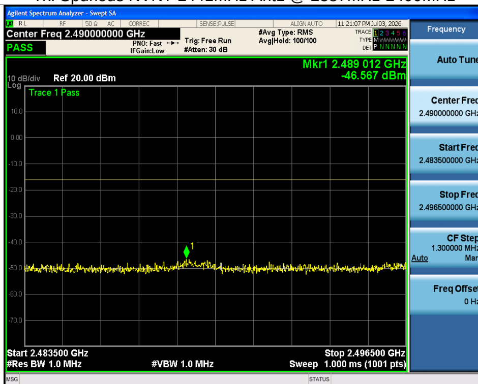
Tx. Spurious NVNT 2441MHz Ant1 @ 2483.5MHz-2496.5MHz
