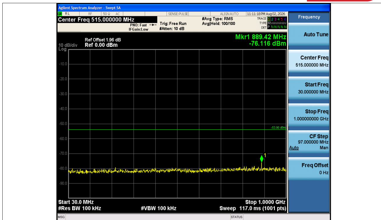
Rx. Spurious NVNT 2441MHz Ant1 @ 30MHz-1000MHz
