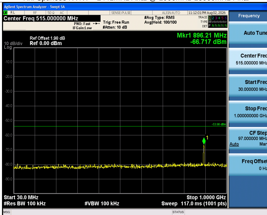
Rx. Spurious NVNT 2480MHz Ant1 @ 30MHz-1000MHz
