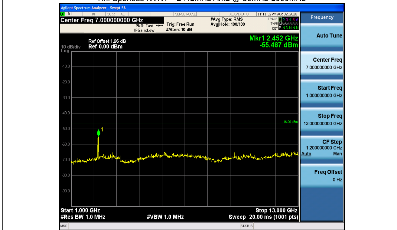
Rx. Spurious NVNT 2441MHz Ant1 @ 1000MHz-13000MHz
