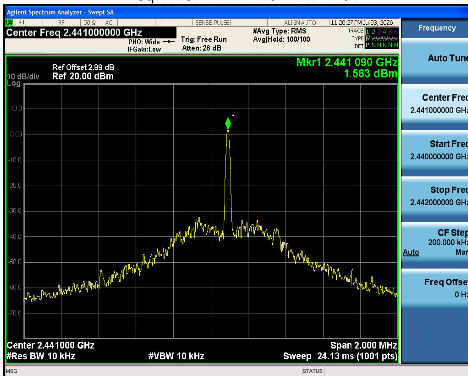
Freq. Error NVNT 2441MHz Ant1
