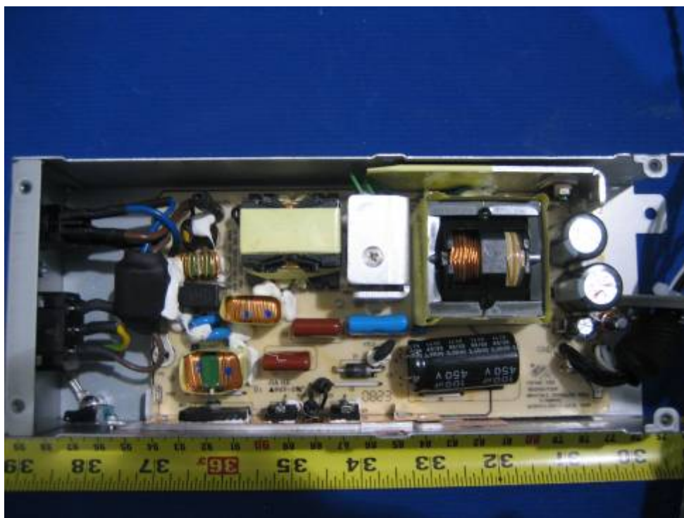
EUT Power Supply – PCBA Component View
