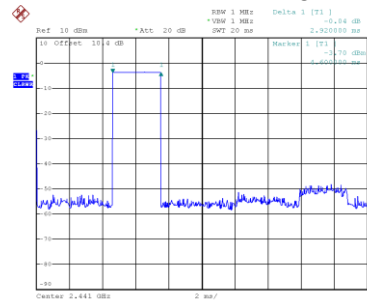
2441MHz-DH5
