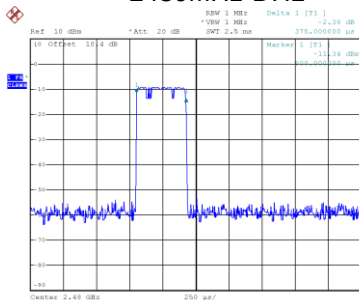
2480MHz-DH1
