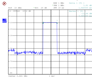
2441MHz-DH3
