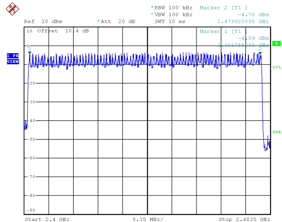
BT (3 Mbps)
