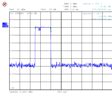
2441MHz-DH1
